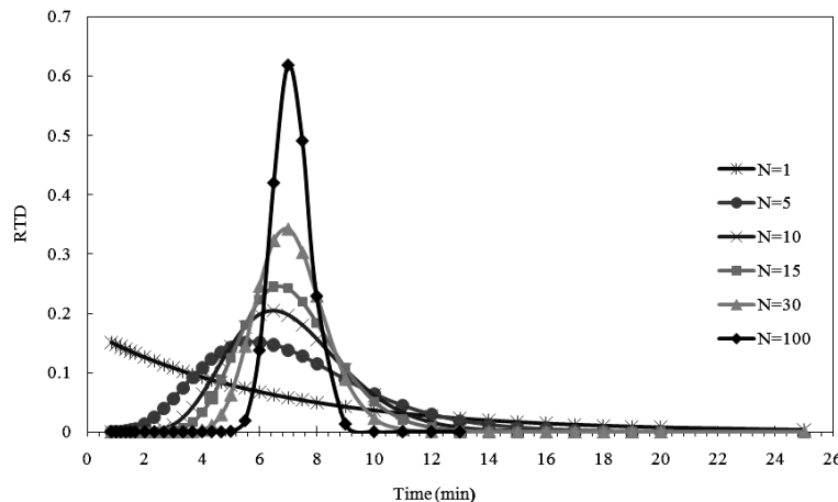
Fig. 5. Effect of the number of perfect mixer containers ( n ) in N-Mixer model on RTD in mixer
