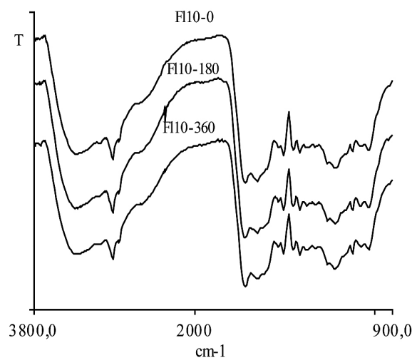
Figure 1. FT-IR of humic acids of Fluvisol
