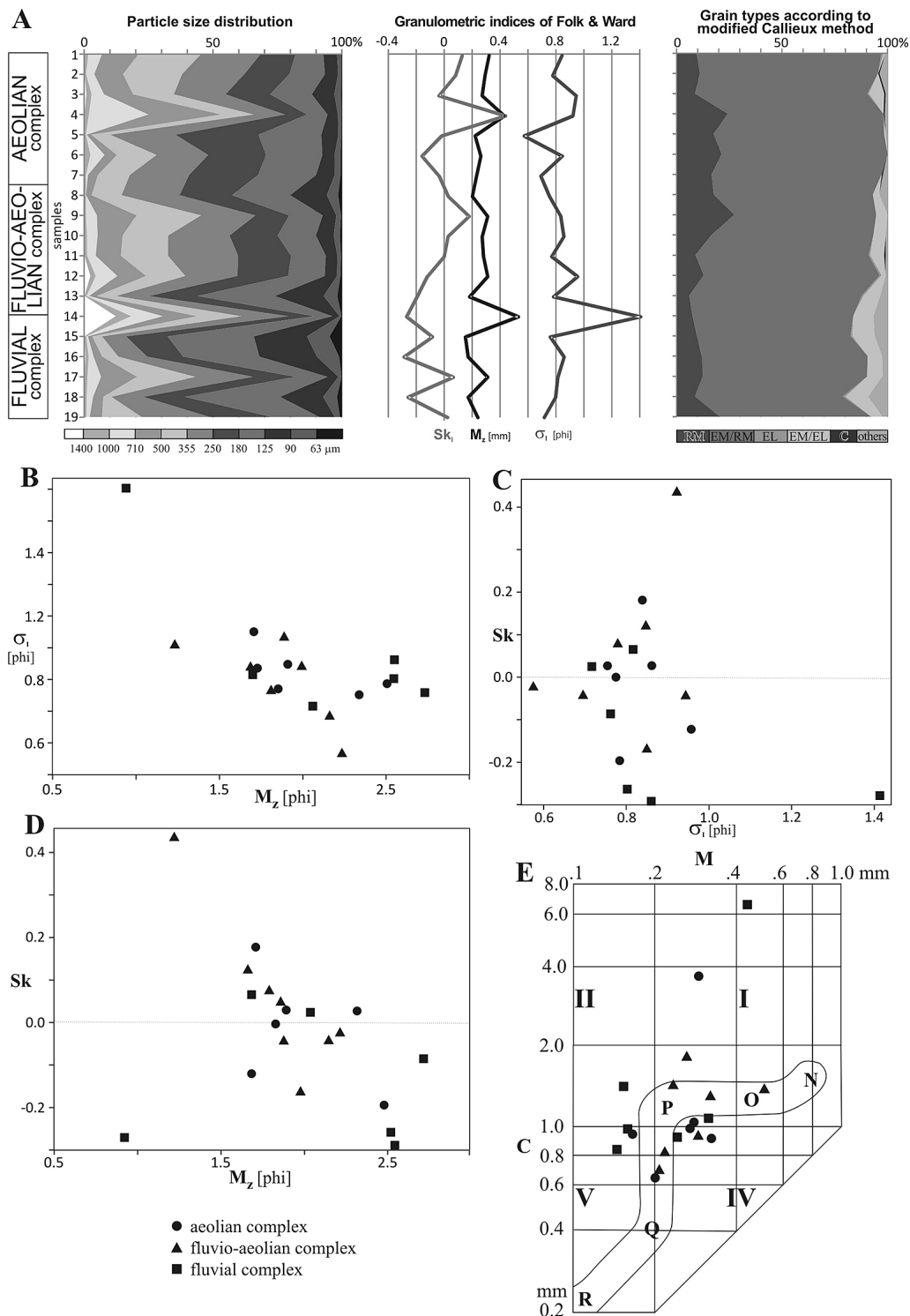
Fig. 4.A – Results of grain-size and morphoscopic analyses at the Postolin section; parameters of grain size distribution after Folk & Ward (1957): mean grain size ( M_z ), sorting ( \sigma_i ), skewness ( Sk_i ); frosting and rounding classes of quartz grains by modified Cailleux's method (Mycielska-Dowgiałło & Woronko, 1998): rounded and frosted grains (RM, rounding degree: 0.7–0.9, following Krumbein, 1941), (2) moderately rounded and frosted grains (EM/RM, rounding degree: 0.3–0.6), rounded and shiny grains (EL, rounding degree: 0.7–0.9), moderately rounded and shiny grains (EM/EL, rounding degree: 0.3–0.6), fresh, angular grains (NU, rounding degree: 0.1–0.2), cracked (C); B-D – Comparison of parameters calculated after Folk and Ward (1957): B – mean grain size ( M_z ) to sorting ( \sigma_i ); C – sorting ( \sigma_i ) to skewness ( Sk_i ); D – mean grain size ( M_z ) to skewness ( Sk_i ); E – Results of grain-size analysis in a CM Passega diagram.
