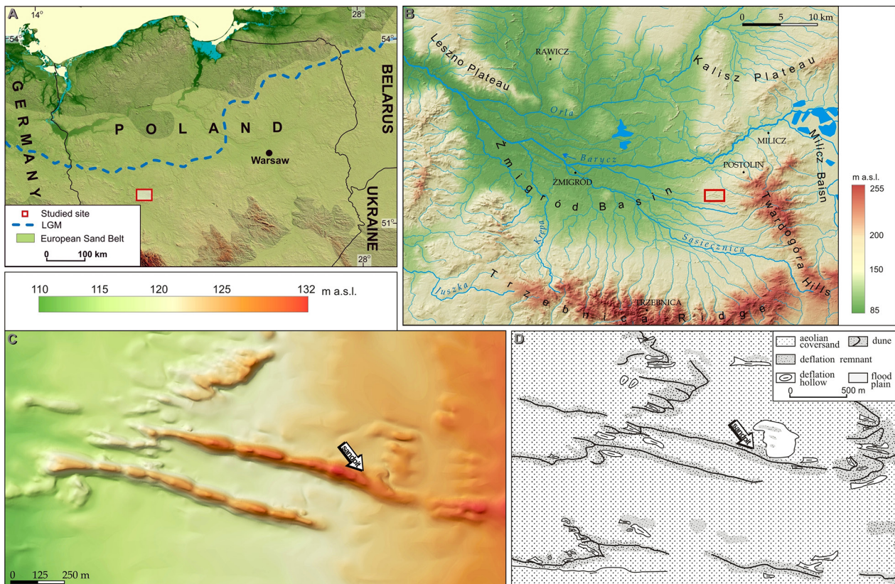
Fig. 1. Location of the study site against the background of: A – The extent of the Sand Belt in central Europe according to Koster (1988) and Kasse (1997); B – DEM of the Żmigród Basin; C – DEM of the study area; D – geomorphological sketch.
