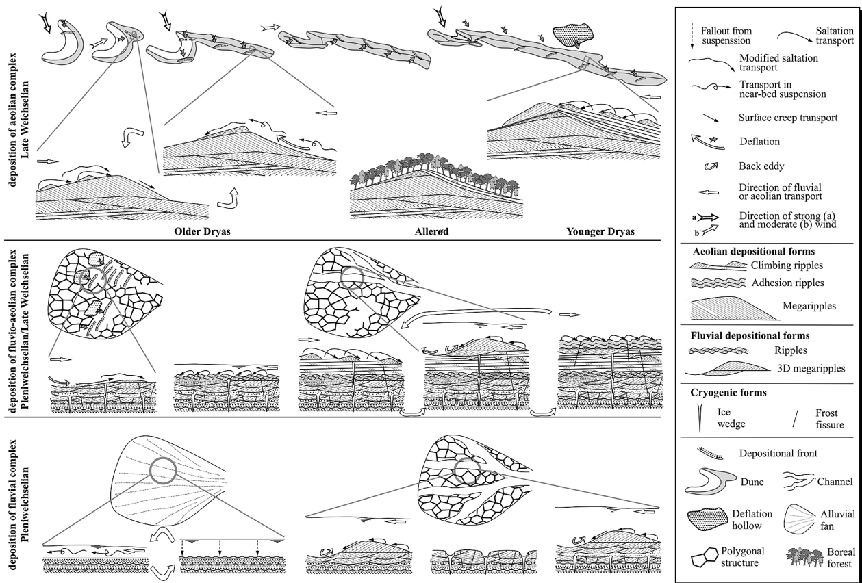
Fig. 5. Model of depositional environments.
