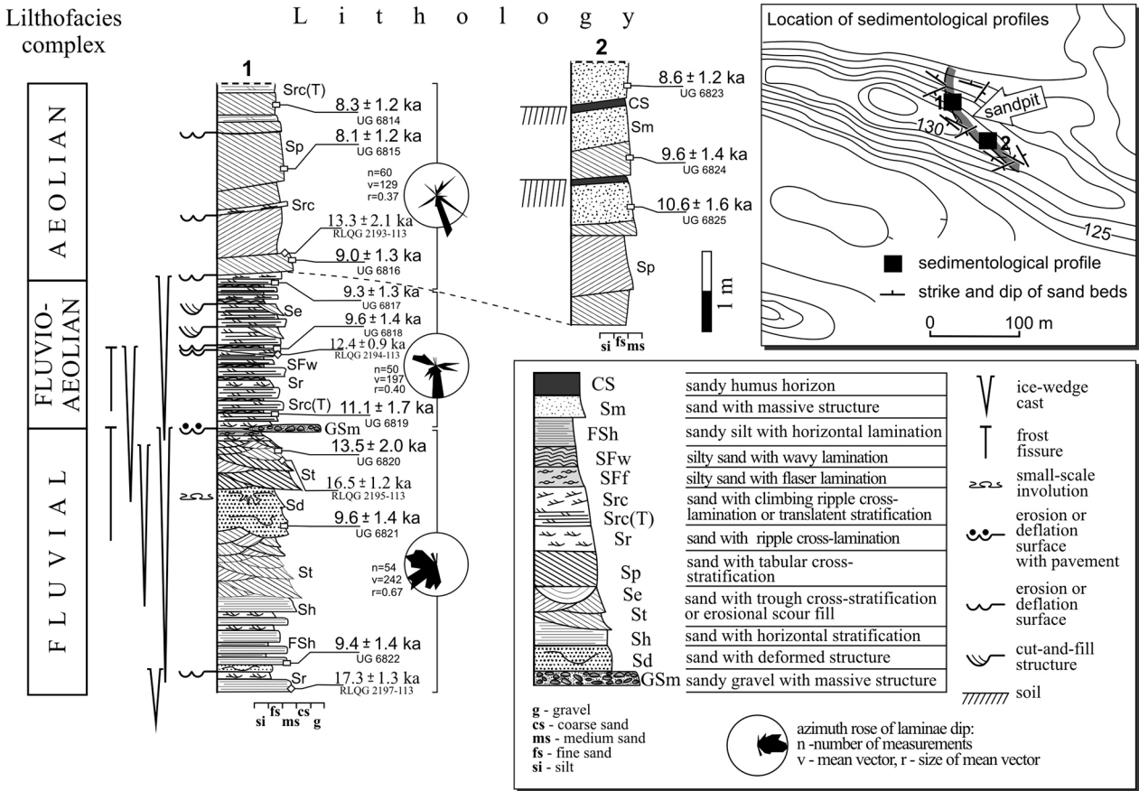
Fig. 2. Sedimentary successions studied.
