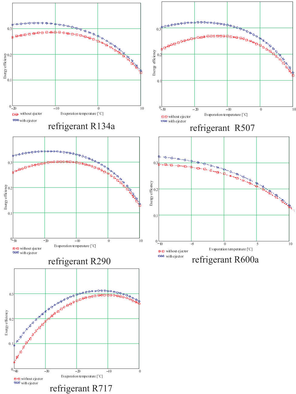
Figure 6. Exergy efficiency vs. temperature of evaporation of ejector-compression and compression refrigeration cycles at condensation temperature t_k = 35\text{ °C} for various working fluids.
