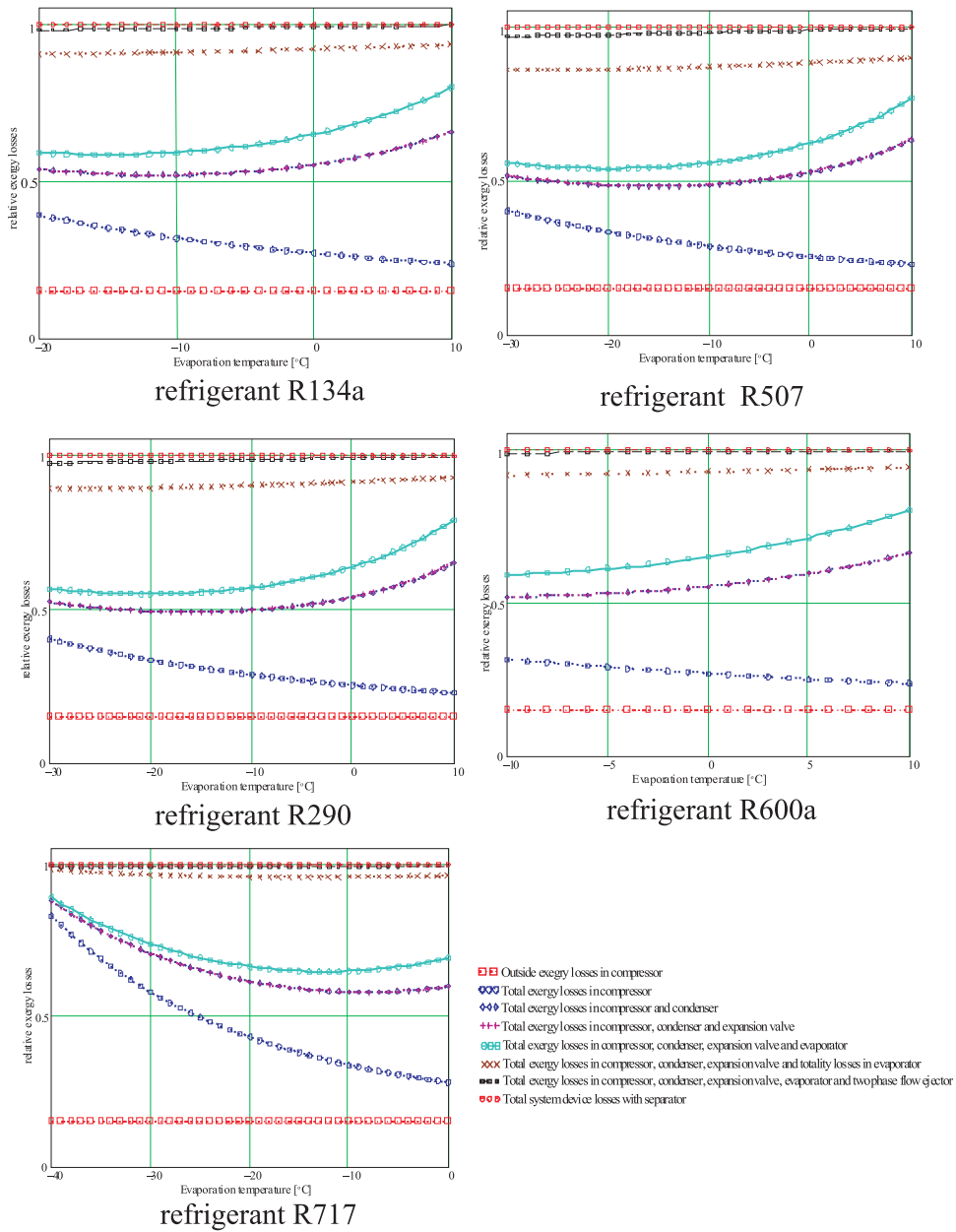
Figure 5. Relative exergy losses of ejector-compression refrigeration cycle vs. temperature of evaporation at condensation temperature t_k = 35\text{ }^\circ\text{C} for various working fluids.
