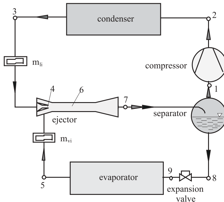
Figure 1. Compression refrigeration system with ejector as a booster compressor.
