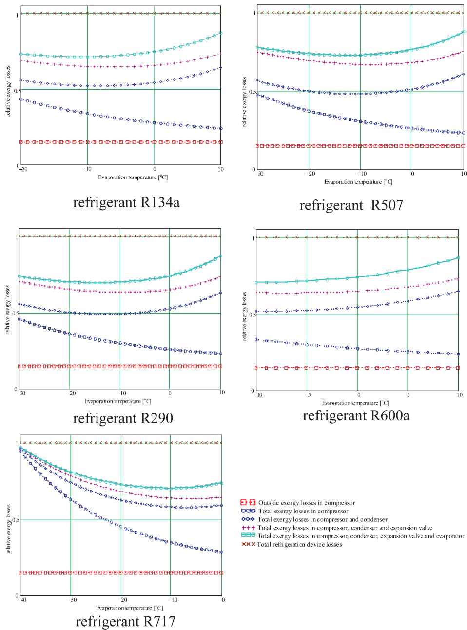
Figure 4. Relative exergy losses of compression refrigeration cycle vs. temperature of evaporation at condensation temperature t_k = 35\text{ }^\circ\text{C} for various working fluids.
