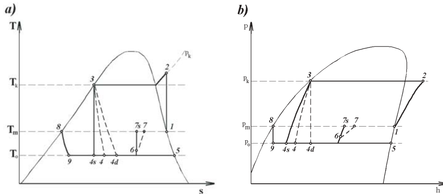
Figure 2. Thermodynamic cycles of ejector-compression system: a) at T-s coordinates, b) at p-h coordinates.
