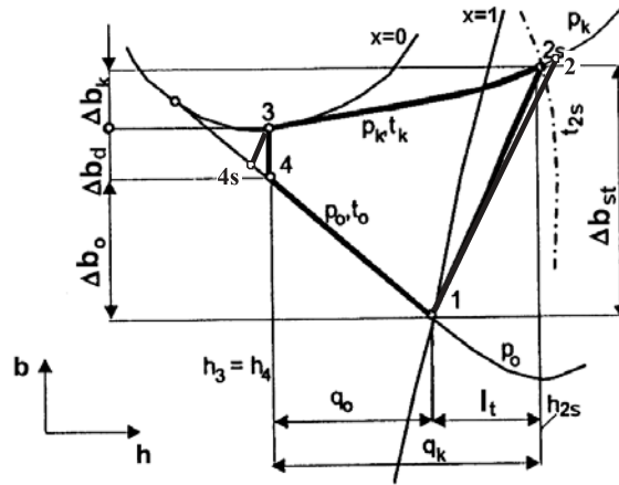
Figure 3. Refrigeration compression cycle in exergy – specific enthalpy ( b - h ) coordinates [18].
