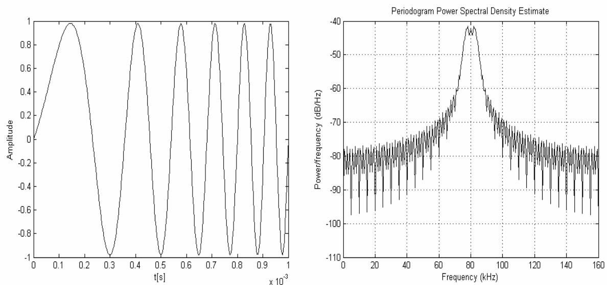
Fig. 1. LFM signal generated in Matlab environment.
