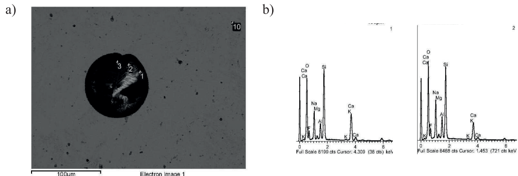
Fig.8. Characteristic non-metallic inclusion from bloom: a) microscopic view, b) chemical compositions
