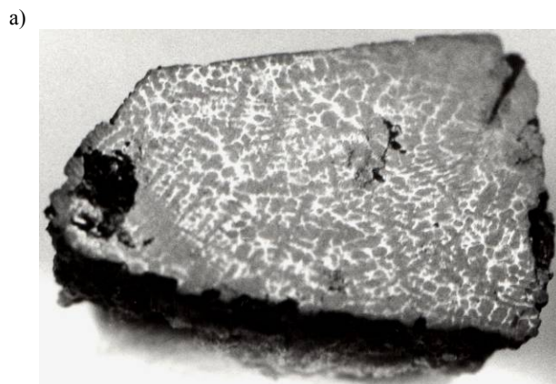
Fig. 1. Non-alloyed cast steel; a) oxidized surface of hot cracks and the shrinkage porosity, magn. 3 \times ; b) the type II sulphides revealed at the surfaces of the intergranular fracture, magn. 250 \times ; c) the type II sulphides, magn. 600 \times
