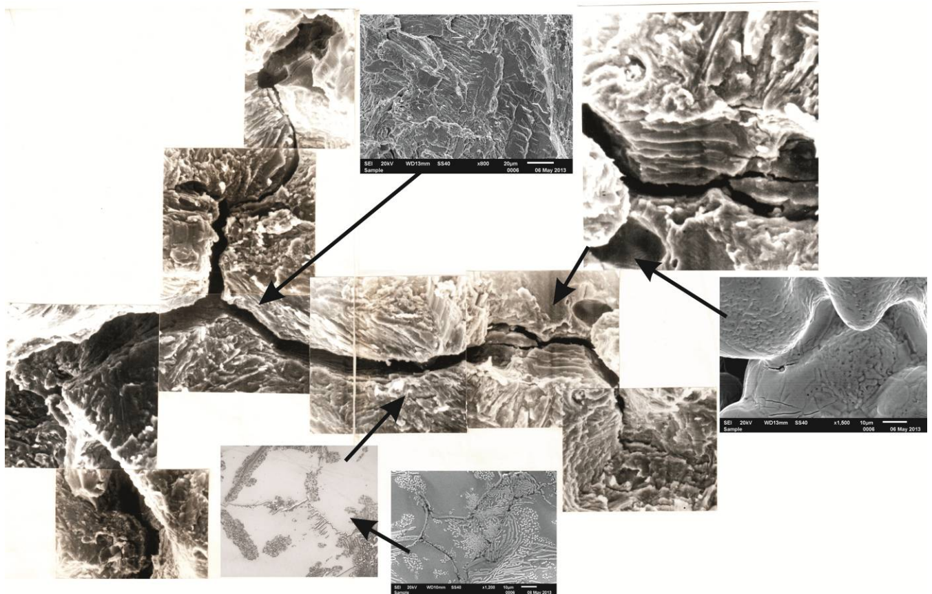
Fig. 4. Hot crack initiated by shrinkage spreading on the boundaries of large grains of solidification and details of eutectics. Scanning microscope
