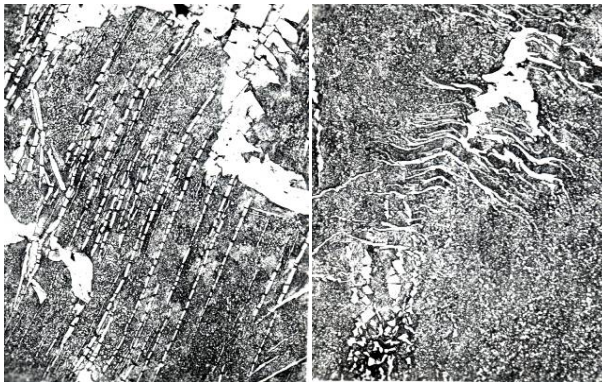
Fig. 3. Deformed and cracked secondary cementite plates in the casting made of L180HMF cast steel, magn. 60 \times , etched with Nital
