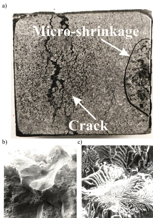
Fig. 1. Non-alloyed cast steel; a) oxidized surface of hot cracks and the shrinkage porosity, magn. 3 \times ; b) the type II sulphides revealed at the surfaces of the intergranular fracture, magn. 250 \times ; c) the type II sulphides, magn. 600 \times
