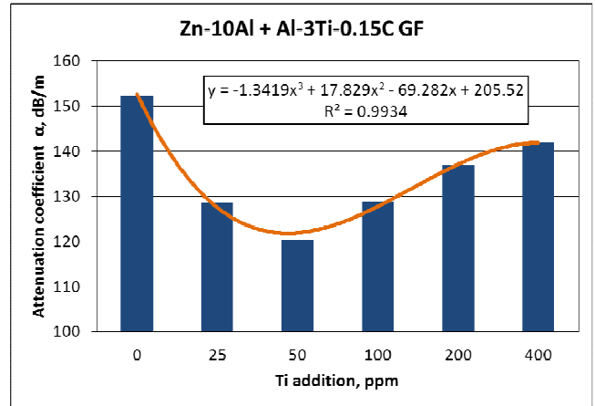
Fig. 2. Summary the effect of the addition of Ti in the Al-3Ti-0.15C (TiCAI) master alloy on the mean value of attenuation coefficient
