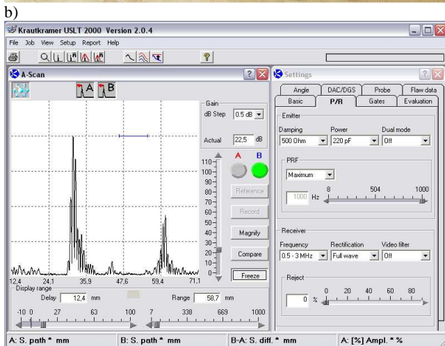
Fig. 1. (a): Krautkramer USLT 2000 stand; (b): Exemplary image of peaks in an echogram of the examined Zn-10Al alloy
