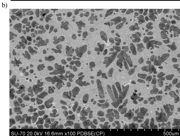
Fig. 5. Changes of microstructure of the Zn-10Al alloy. (a) initial alloy without Ti addition, (b) the same alloy doped with 100 ppm Ti introduced with the Al-3Ti-0.15C grain refiner, SEM [6]
