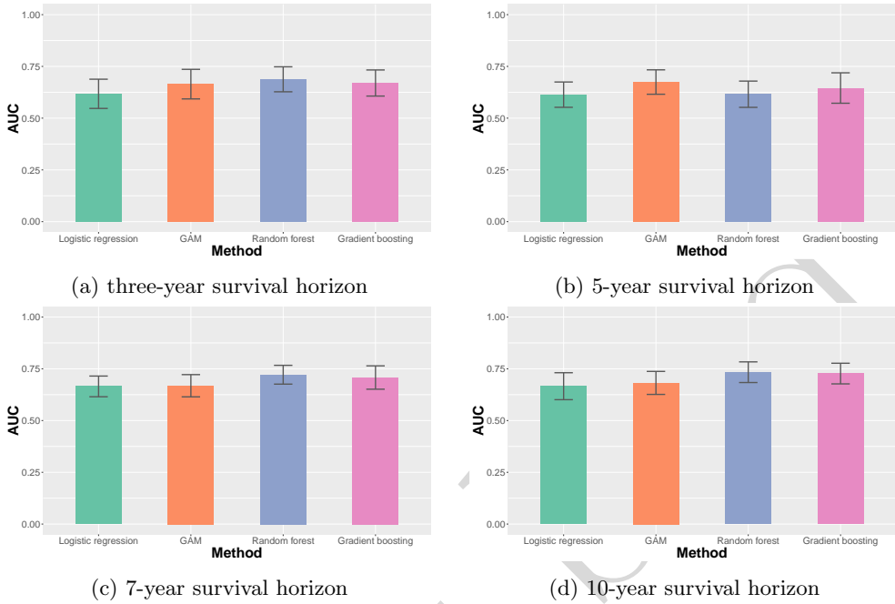
Figure 5. Classifier AUC results with standard deviation (error bars on top of each bar) for various methods across different survival horizons. On each subfigure, bars represent machine-learning methods (starting from left): logistic regression (green); GAM (orange); random forest (blue); and gradient boosting (purple).
