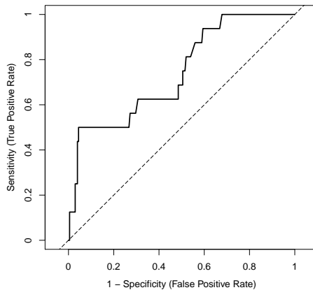
Figure 4. ROC curve (black line) with AUC of 0.7421 for random forest model for three-year survival time horizon. Dashed line represents baseline ROC curve.
