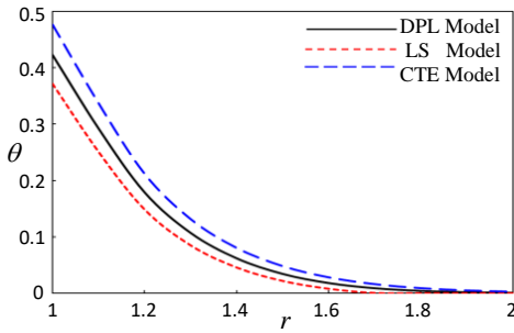
Fig. 1. Temperature distribution \theta for different values of phase-lags \tau_q and \tau_\theta
