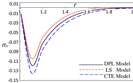
Fig. 3. Thermal stress distribution \sigma_{rr} for different values of phase-lags \tau_q and \tau_\theta
