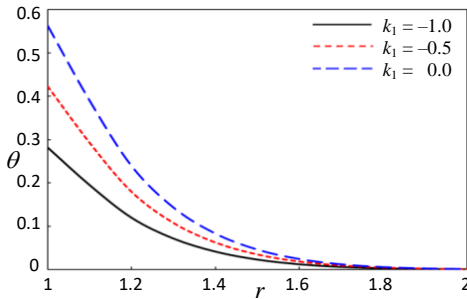
Fig. 5. Temperature distribution \theta for different values of thermal conductivity parameter k_1
