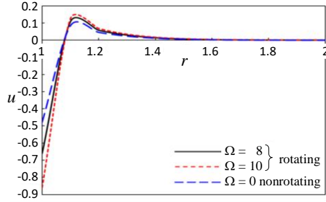
Fig. 10. Displacement distribution u for different values of angular velocity (rotation) \Omega
