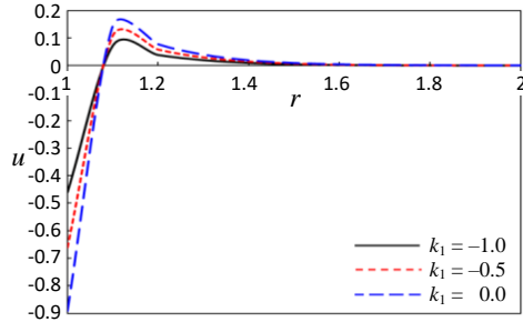
Fig. 6. Displacement distribution u for different values of thermal conductivity parameter k_1
