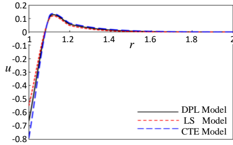
Fig. 2. Displacement distribution u for different values of phase-lags \tau_q and \tau_\theta
