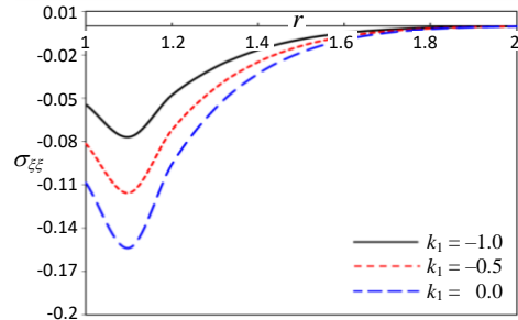
Fig. 8. Thermal stress distribution \sigma_{\xi\xi} for different values of thermal conductivity parameter k_1
