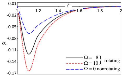
Fig. 11. Thermal stress distribution \sigma_{rr} for different values of angular velocity (rotation) \Omega
