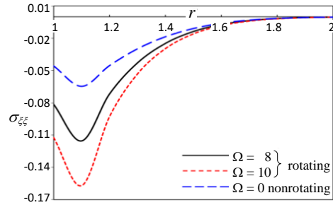
Fig. 12. Thermal stress distribution \sigma_{\xi\xi} for different values of angular velocity (rotation) \Omega
