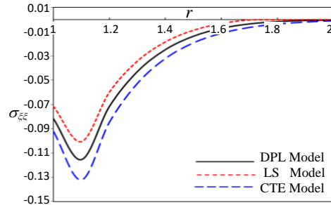
Fig. 4. Thermal stress distribution \sigma_{\xi\xi} for different values of phase-lags \tau_q and \tau_\theta
