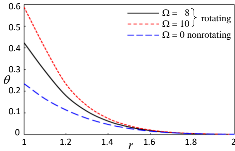
Fig. 9. Temperature distribution \theta for different values of angular velocity (rotation) \Omega
