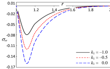
Fig. 7. Thermal stress distribution \sigma_{rr} for different values of thermal conductivity parameter k_1
