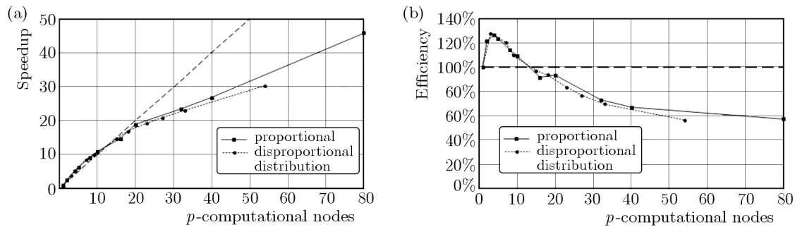
Fig. 12. The results of scalability tests from the first research: (a) speedup and (b) efficiency parameters
