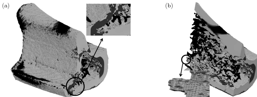
Fig. 11. (a) FEM simulation results of the rat bone model (Strain Energy Density distribution: black color – no energy; dark grey – high energy regions) and (b) the cross-section of the grid with an enlarged part
