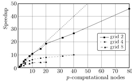
Fig. 13. Mesh generation walltime for the proportional and the disproportional distribution slices per domains
