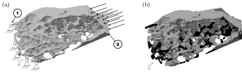
Fig. 10. (a) Boundary conditions applied to the test case (1 – fixed plane, 2 – pressure force applied to cortical bone) and (b) results of FEM simulation (Strain Energy Density distribution: black color – no energy; dark grey – high energy regions)
