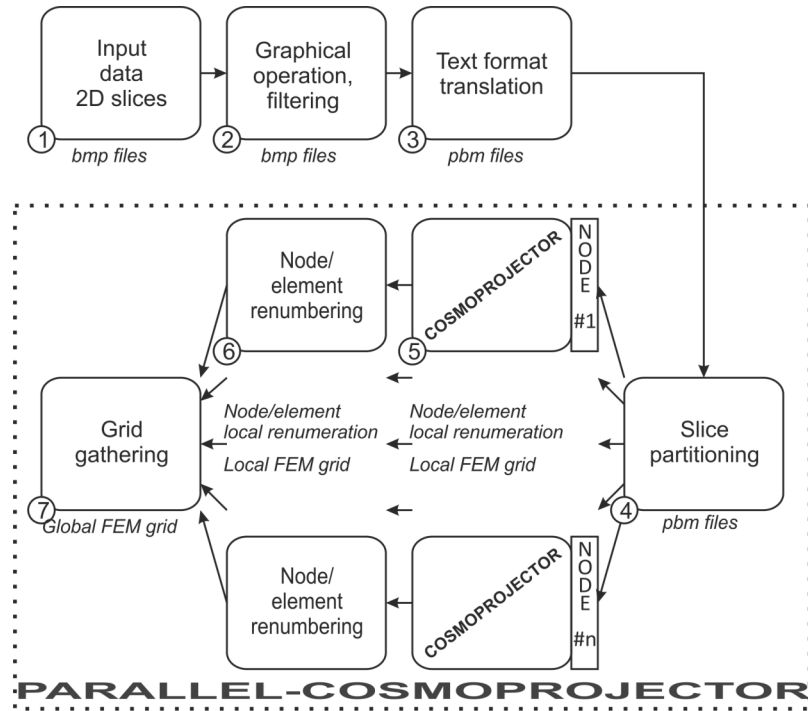
Fig. 6. The parallel mesh generator – Parallel-Cosmoprojector
