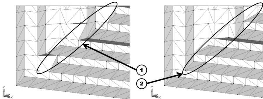
Fig. 7. The grid (1) without overlaps at the boundary of the subdomains causes incorrect geometry representation in opposition to the grid (2) created by assembling of subdomains with the overlaps
