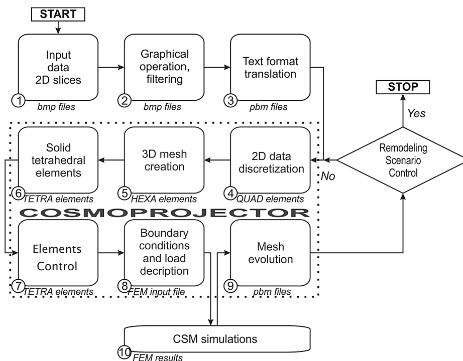
Fig. 1. The scheme of a biomimetic optimization system where the mesh generator – Cosmoprojector – is the essential part (dash line) (Nowak, 2006b)
