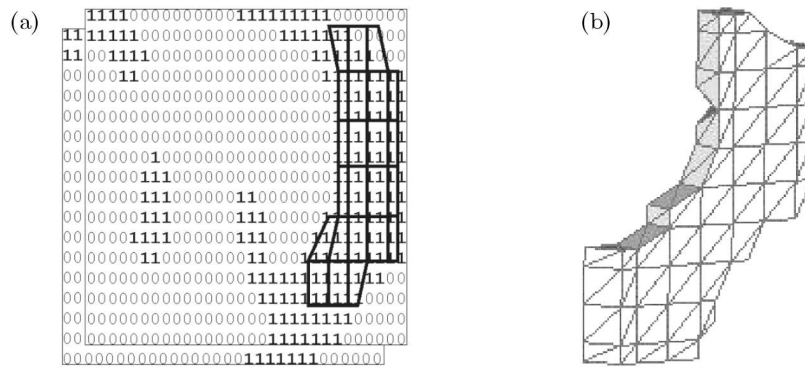
Fig. 3. The discretization of input data: (a) division of images into QUAD elements and (b) the projection of QUAD elements into adjacent slices – generating HEXA elements and their division into TETRA elements
