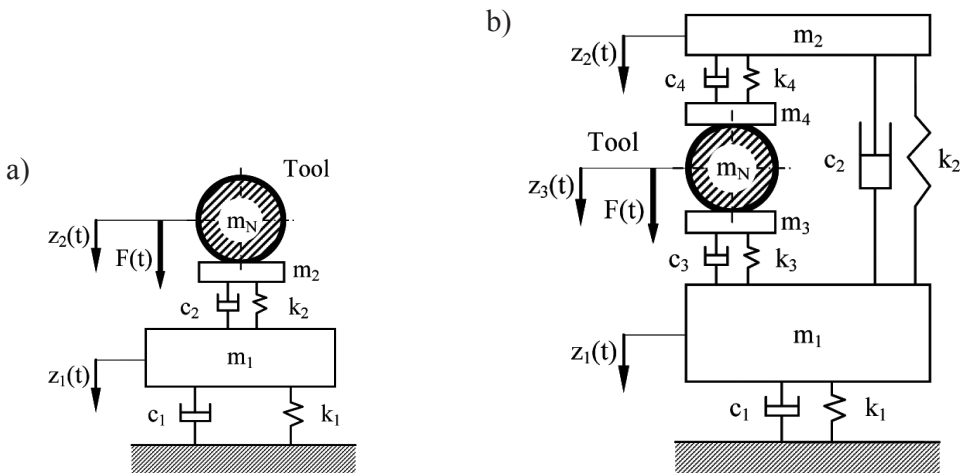
Fig. 1. A synthesis of the ISO 10068:2012-based human physical models and the tool model: a) model 1 – annex B; b) model 2 – annex C [13]
