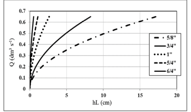
Fig. 3. Relationship between discharge Q and head loss hL ( n = 3 , R : D = 2 ) with Equation 11; source: own study
