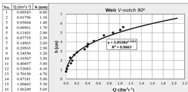
Fig. 7. Discharge Q validation of weir V-notch 90°; source: own study
