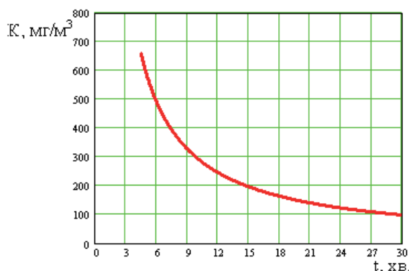
Fig. 3. The dependence of time of exposure at various concentrations of ozone, which is necessary to ensure 2940 mg dose processing of \text{m}^3/\text{min}
