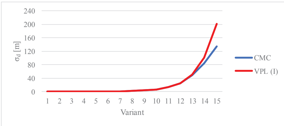
Fig. 3. Standard deviation of distance \sigma_d computed by VPL (I) and CMC estimate \hat{\sigma}_d for correlated coordinates ( \rho_{X_A, Y_A} = 0.5, \rho_{X_B, Y_B} = 0.5 )
