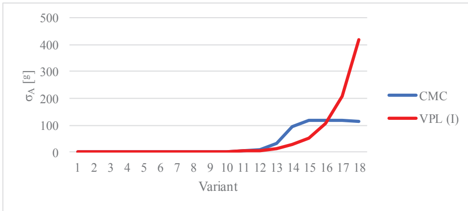
Fig. 5. Standard deviation of azimuth \sigma_A computed by VPL (I) and CMC estimate \hat{\sigma}_A for correlated coordinates ( \rho_{X_A, Y_A} = 0.5 , \rho_{X_B, Y_B} = 0.5 )
