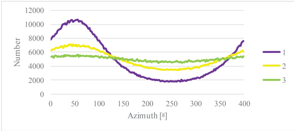
Fig. 6. Histograms of azimuths computed by Crude Monte Carlo method
