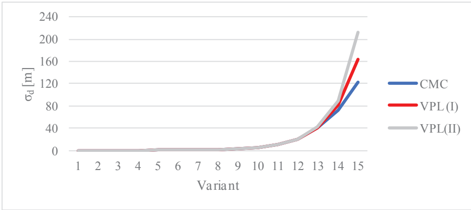
Fig. 2. Standard deviation of distance \sigma_d computed by VPL and CMC estimate \hat{\sigma}_d for uncorrelated coordinates
