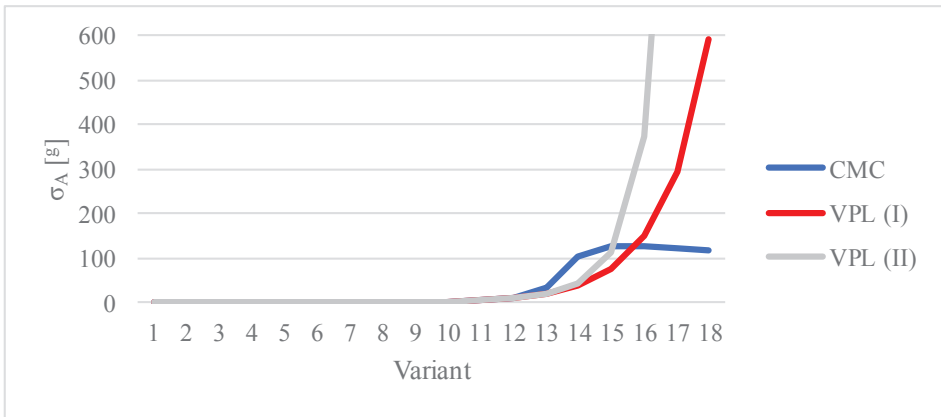
Fig. 4. Standard deviation of azimuth \sigma_A computed by VPL and CMC estimate \hat{\sigma}_A for uncorrelated coordinates
