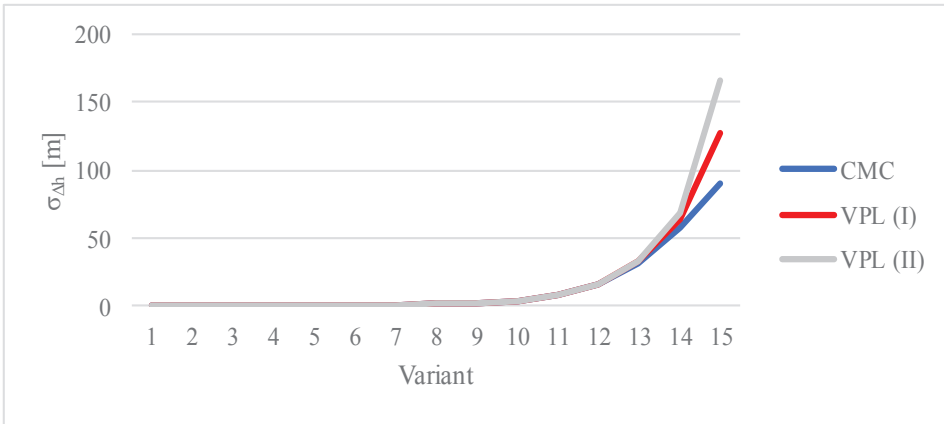
Fig. 1. Standard deviation of height difference in trigonometric levelling \sigma_{\Delta h} computed by VPL (VPL (I) concerns the first-order Taylor series expansion and VPL (II) – the second-order Taylor series expansion) and CMC estimate \hat{\sigma}_{\Delta h}
