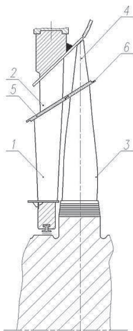
Figure 1. Two-tier stage.
