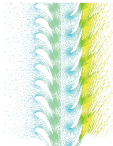
Figure 6. Velocity fields in lower tier of two-tier stage.
