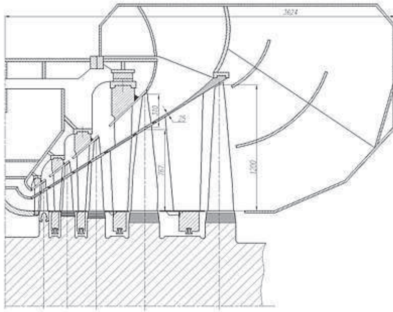
Figure 4. Two-tier low pressure cylinder.
