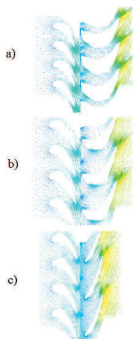
Figure 5. Velocity fields in lower tier of two-tier stage.
