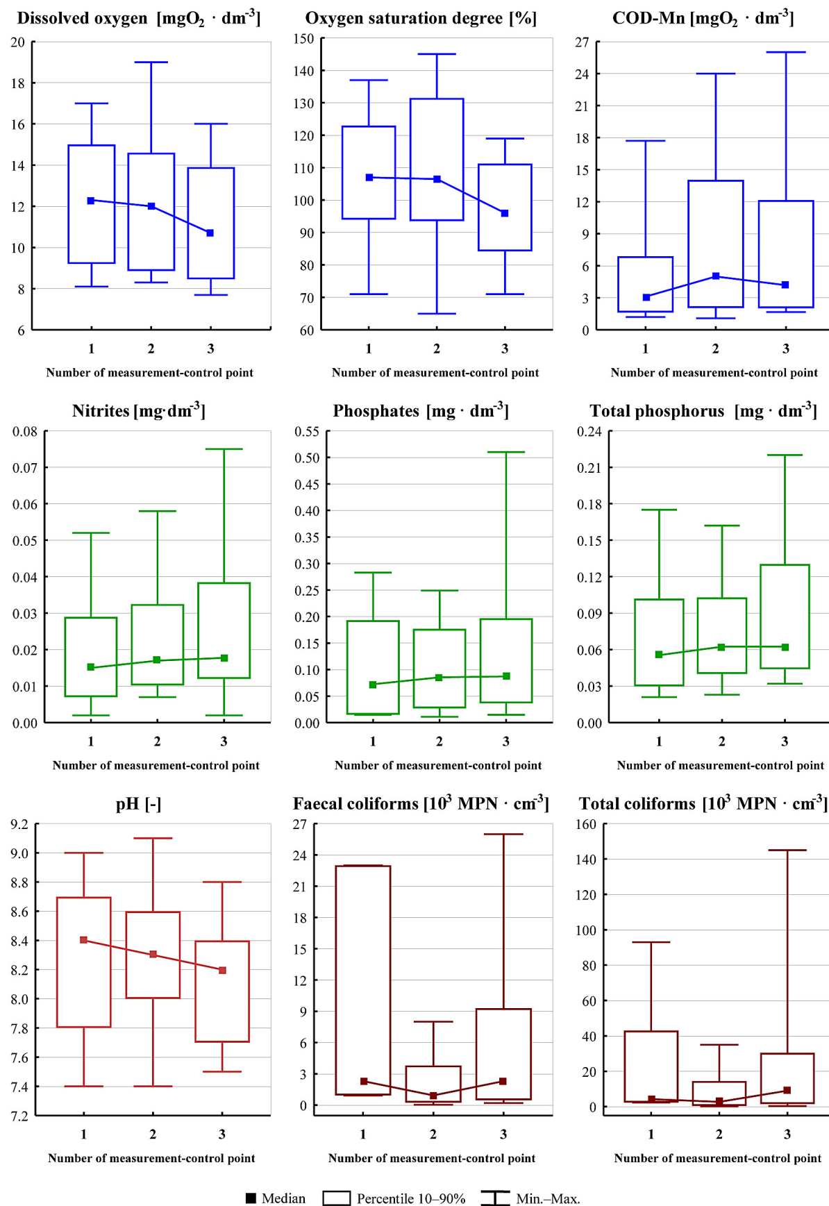
Figure 3. Variability of selected water quality indices along the analyzed Poprad river reach
