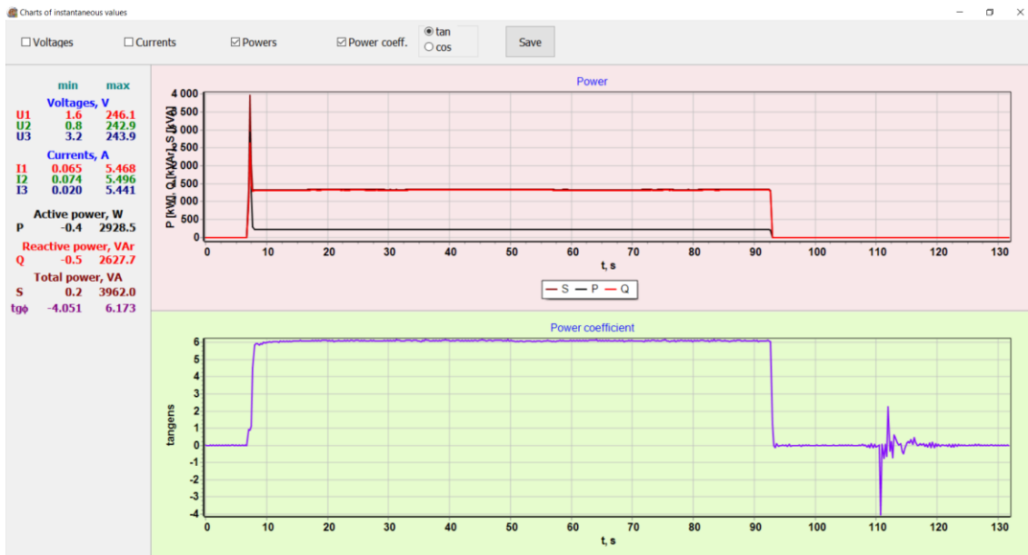
Fig. 8. The diagram of changes in active, passive, apparent power consumption and tgφ power factor in supply system of a model vibratory unit without the inverter at the frequency of 50 Hz
