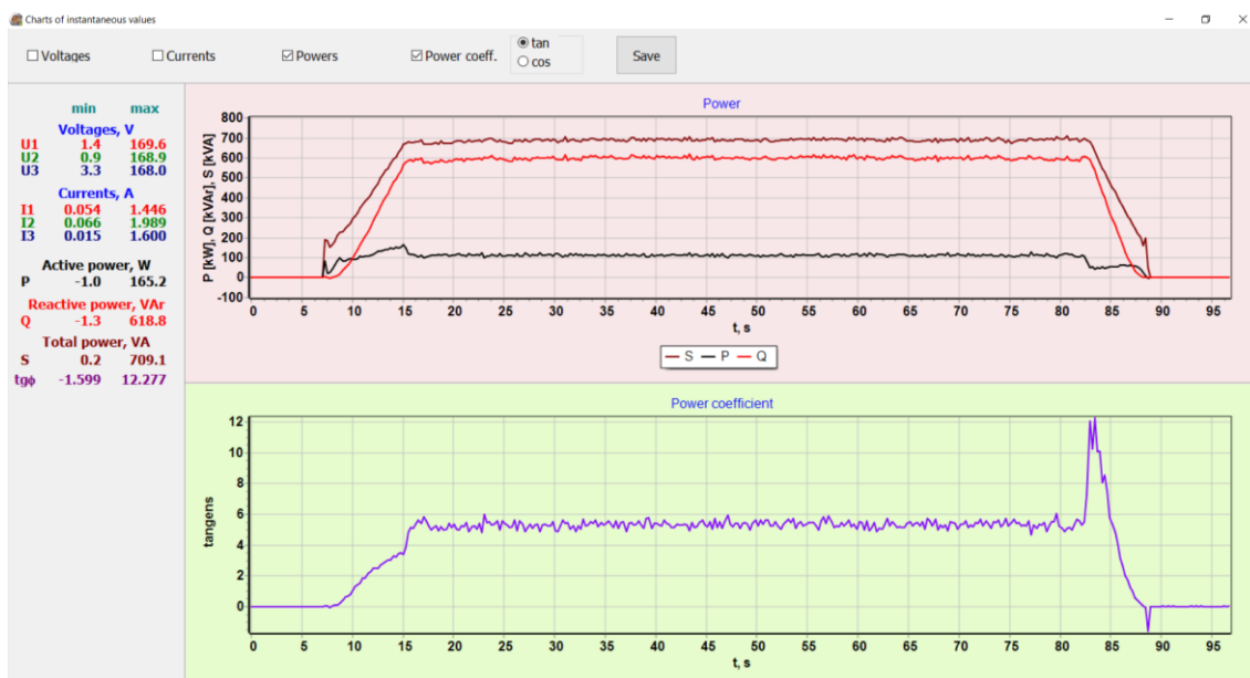
Fig. 5. The diagram of active, passive and apparent power values and tg\phi power factor in the supply system of a model vibratory unit for the inverter output frequency set at 40 Hz
