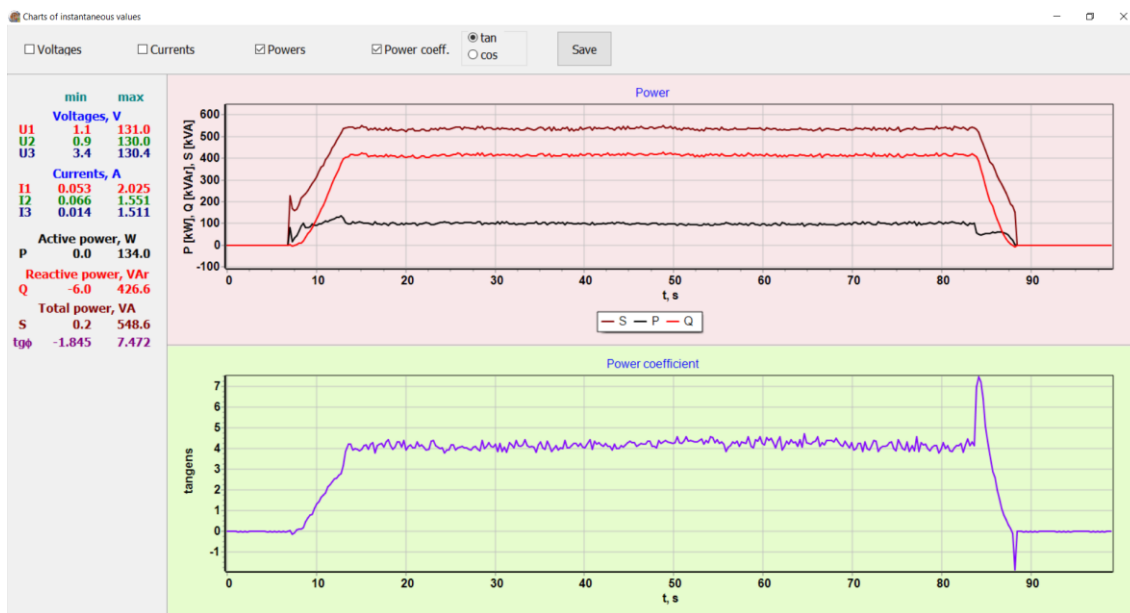
Fig. 4. The diagram of active, passive and apparent power values and tg\phi power factor in the supply system of a model vibratory unit for the inverter output frequency set at 30 Hz
