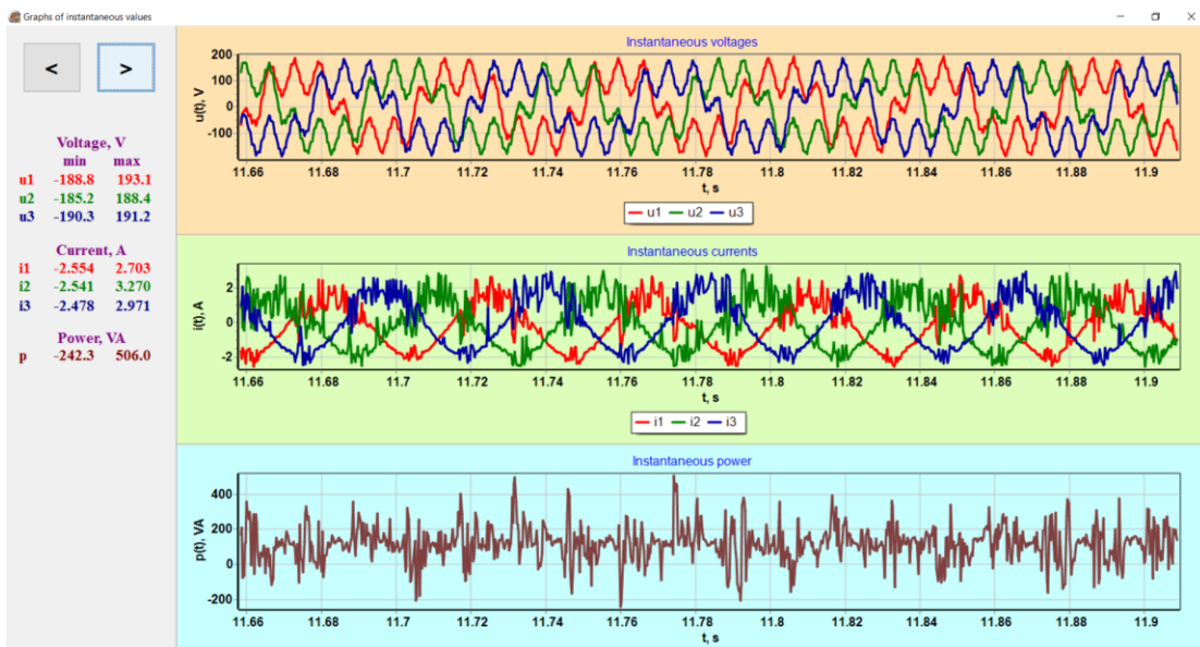
Fig. 3. The recorder’s software window, which includes graphs of changes in instantaneous voltages and currents in the given measurement time-boxed window for a frequency inverter set at a frequency of 30 Hz
