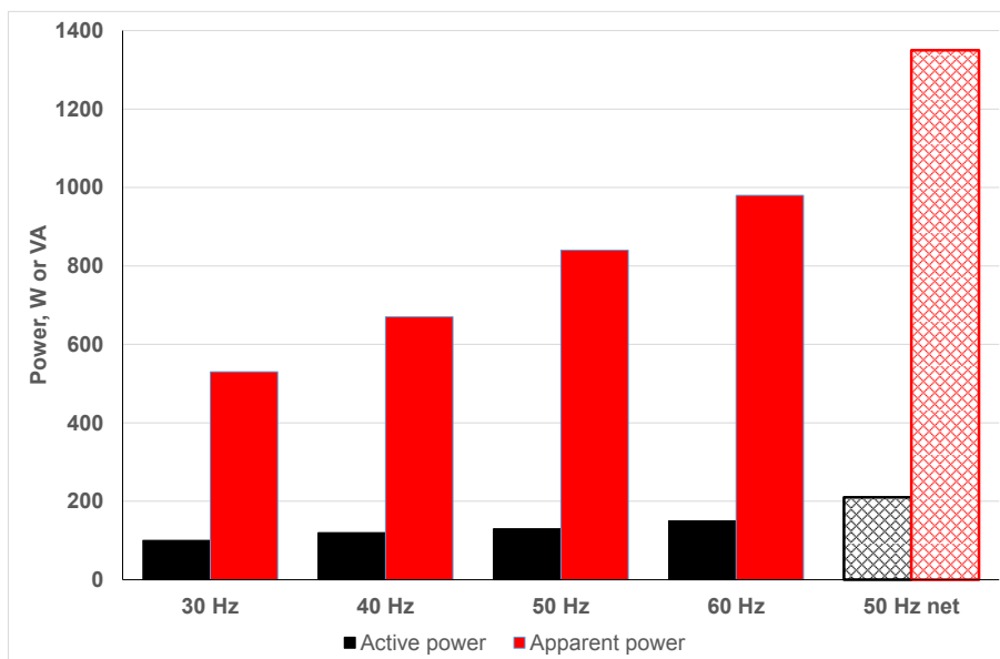
Fig. 9. Diagram of changes in active and apparent power consumption of supply system of model vibratory unit with and without the inverter
