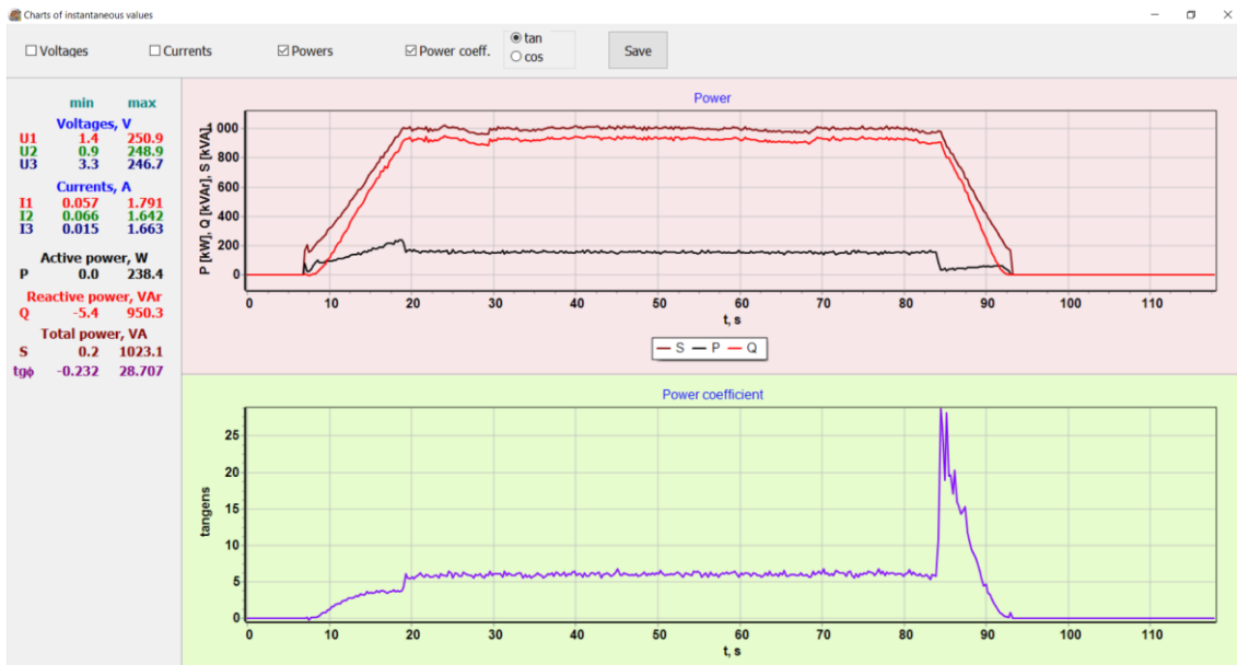
Fig. 7. The diagram of active, passive and apparent power values and \text{tg}\phi power factor in the supply system of a model vibratory unit for the inverter output frequency set at 60 Hz
