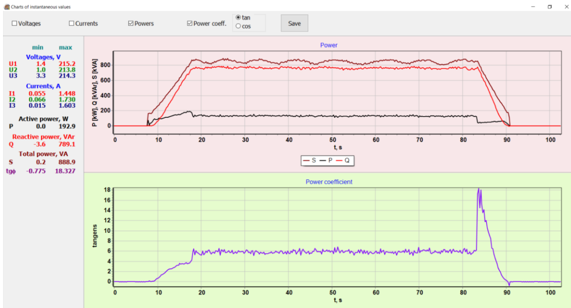
Fig. 6. The diagram of active, passive and apparent power values and \text{tg}\phi power factor in the supply system of a model vibratory unit for the inverter output frequency set at 50 Hz
