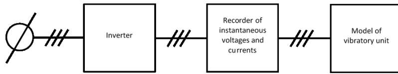
Fig. 1. The recording system of instantaneous voltages and currents values between inverter and model vibratory unit
