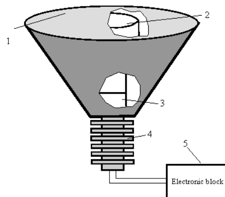
Fig. 2. Schematic representation of the non-contact heat flow meter: 1 – the receiver plate; 2 – the thermoelectric battery heat flow converter; 3 – the thermoelectric cooler; 4 – the radiator; 5 – the signal conditioning and measuring electronics assembly
