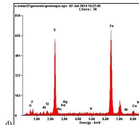
Fig. 5. Microstructures and energy-dispersive spectra of the Akbastau ore: a, c - after mechanical crushing; b, d - after electric pulse reduction
