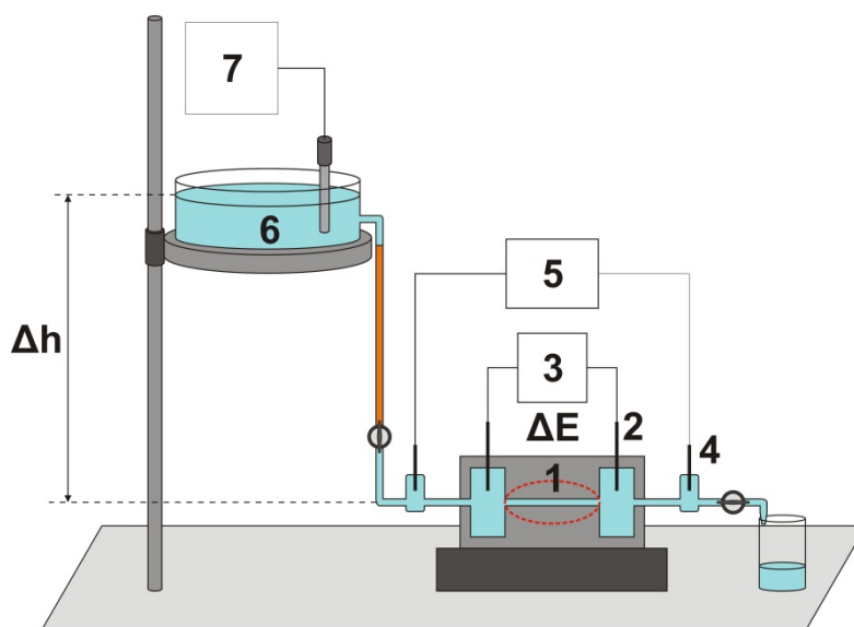
Fig. 1. A schematic view of the parallel-plate channel cell used for streaming potential measurements of bare surfaces of PTFE: 1) electrokinetic cell; 2) AgCl electrodes for streaming potential measurements; 3) streaming potential measurement set-up (electrometer); 4) electrodes for cell resistance measurements; 5) resistance measurement set-up (electrometer and resistor) 6) electrolyte reservoir 7) conductometer (Morga et al., 2016)
