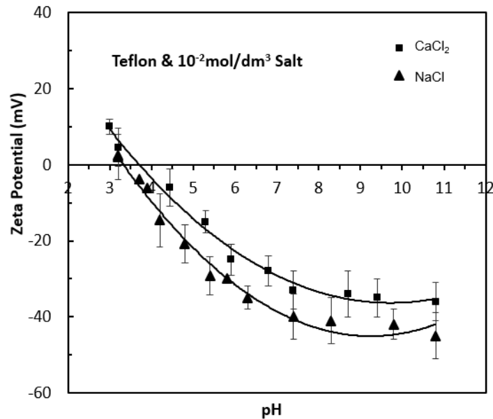
Fig. 5. Zeta potential-pH profiles of Teflon at 1.10^{-2} mol/dm 3 CaCl 2 and NaCl solutions
