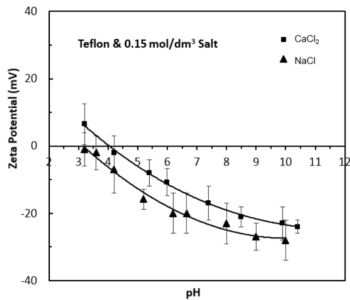
Fig. 6. Zeta potential-pH profiles of Teflon at 0.15 mol/dm 3 CaCl 2 and NaCl solutions
