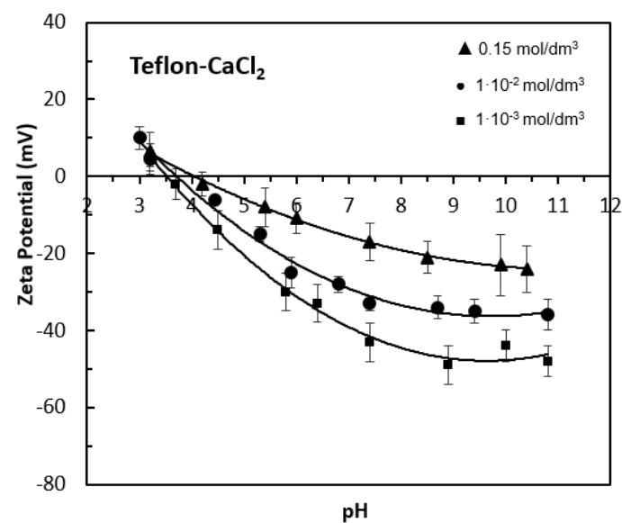
Fig. 3. Zeta potential-pH profiles of Teflon as a function of CaCl 2 concentration ( 1.10^{-3} mol/dm 3 , 1.10^{-2} mol/dm 3 , and 0.15 mol/dm 3 )
