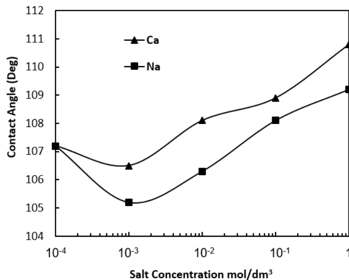
Fig. 7. Contact angles of the plate Teflon as a function of salt concentration
