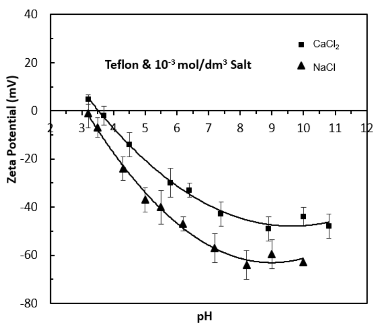
Fig. 4. Zeta potential-pH profiles of Teflon at 1.10^{-3} mol/dm 3 \text{CaCl}_2 and NaCl solutions
