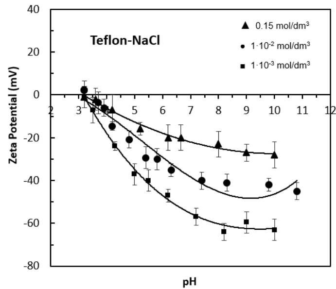
Fig. 2. Zeta potential-pH profiles of Teflon as a function of NaCl concentration ( 1.10^{-3} mol/dm 3 , 1.10^{-2} mol/dm 3 , and 0.15 mol/dm 3 )
