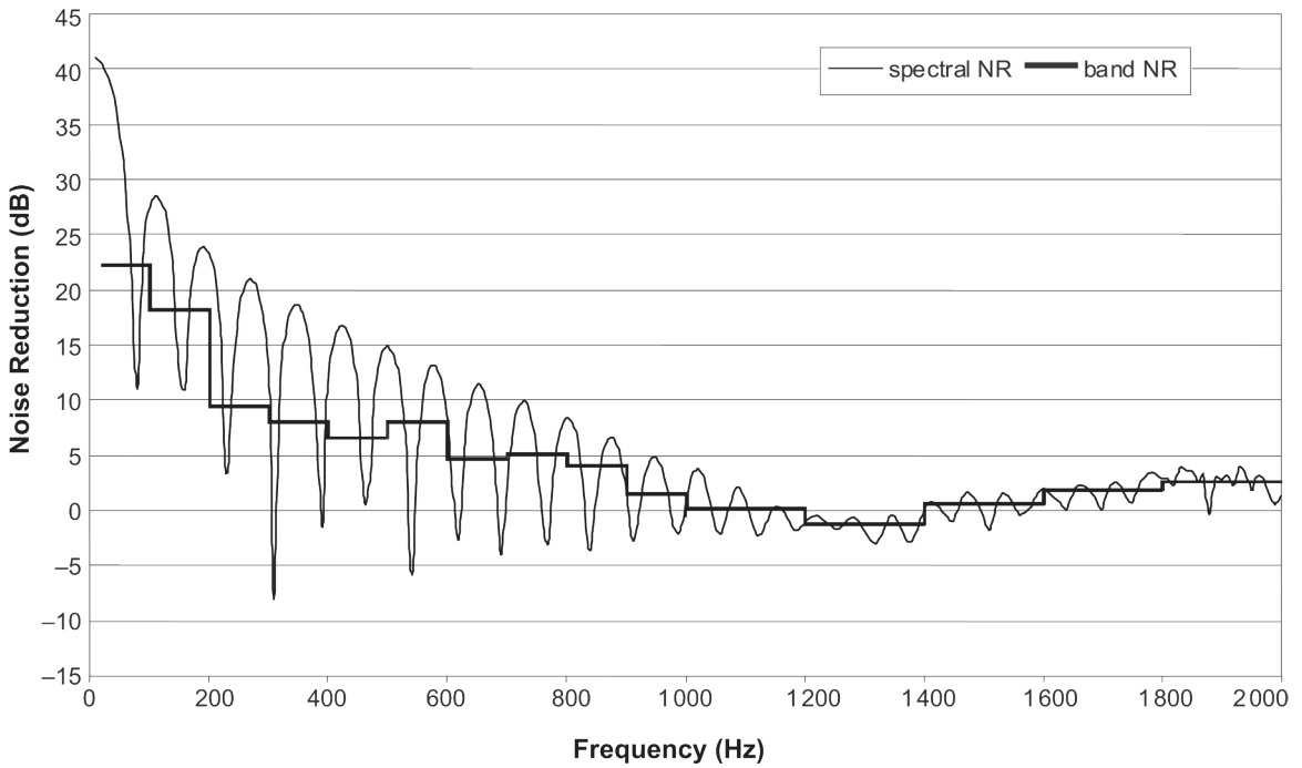
Figure 10. Spectral and band noise reduction (NR) for 9 spiral leads in a tube 1 m in length.
