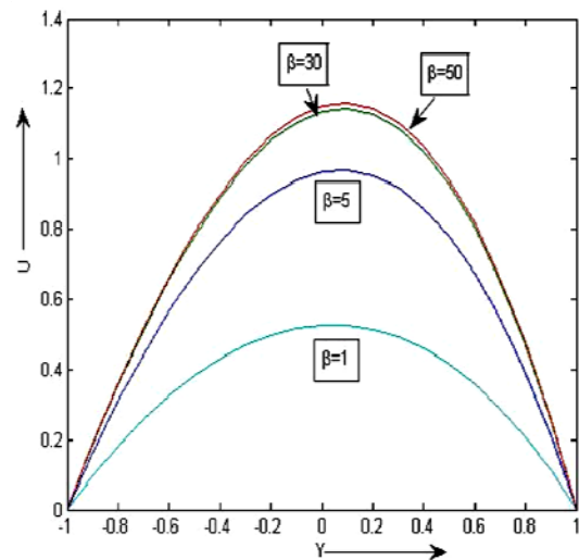
Fig.2. U versus Y for various non-Newtonian parameter values ( \beta ) at t = 0.5 .
