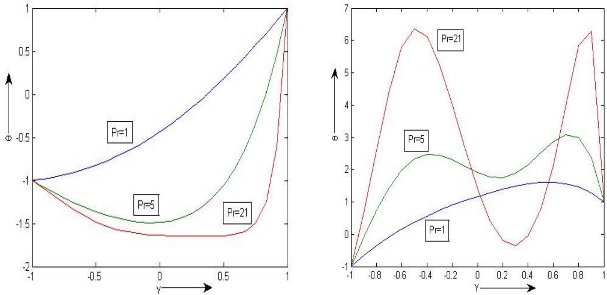
Fig.6. \theta versus Y for different values of Pr at t = 0.5 for two Eckert numbers (a) Ec=6 \times 10^9 (b) Ec=0.006 .
