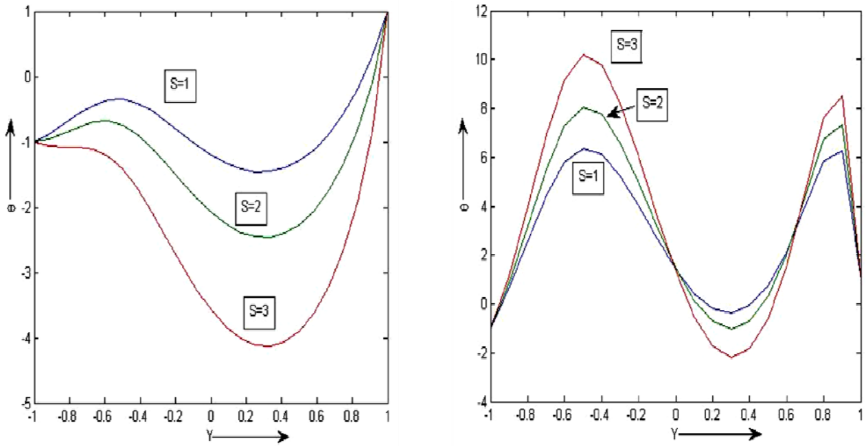
Fig.8. \theta versus Y for various source parameter values ( S ) at t = 0.5 for two Eckert numbers Ec=0.0006 (a) Ec=0.006 .
