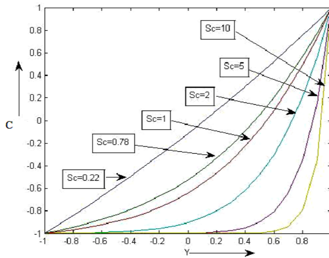
Fig.9. Concentration versus Y for various Schmidt numbers ( Sc ) at t = 0.5 .
