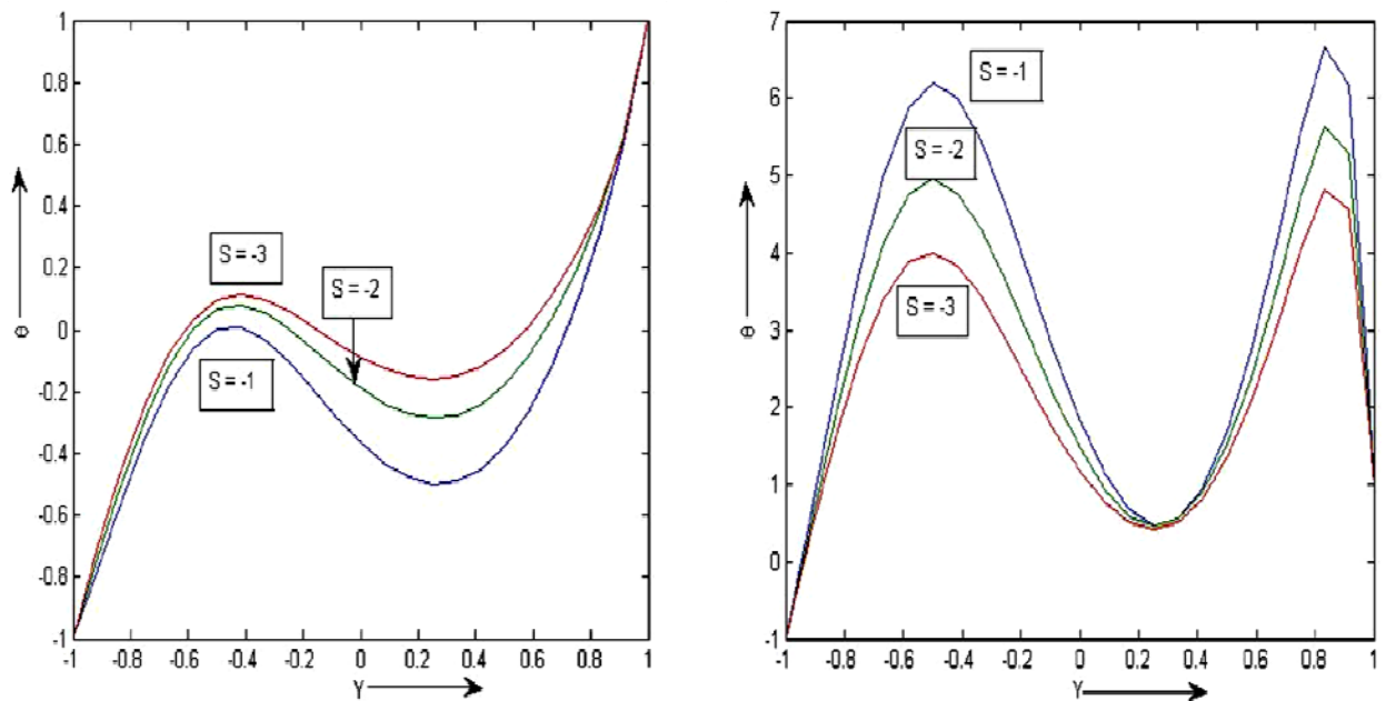
Fig.7. \theta versus Y for various sink parameter values( S ) at t = 0.5 for two Eckert numbers (a) Ec=0.0006 (b) Ec=0.006 .
