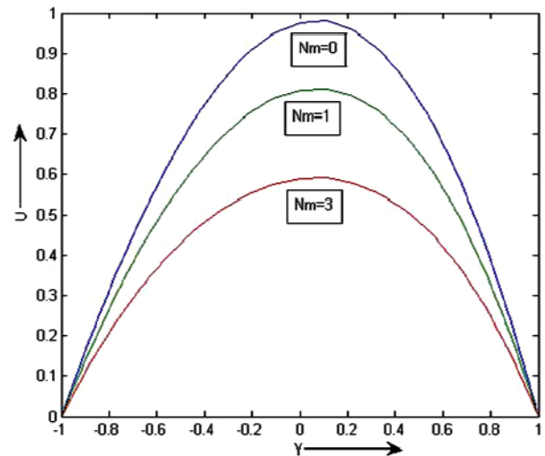
Fig.4. U versus Y for various hydromagnetic parameter values ( Nm ) at t = 0.5 .
