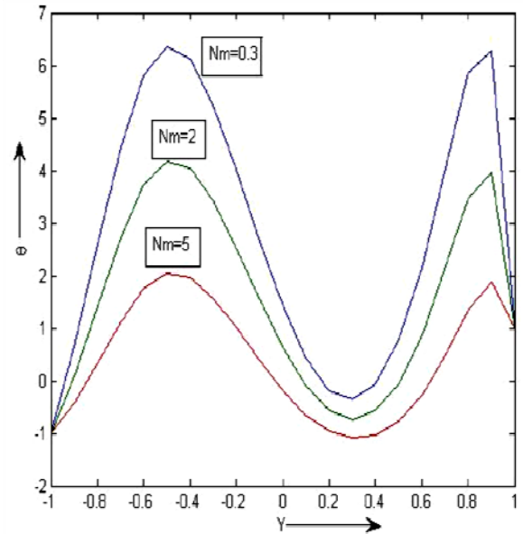
Fig.5. \theta versus Y for various hydromagnetic parameter values ( Nm ) at t = 0.5 for two Eckert numbers (a) Ec=0.0006 (b) Ec=0.006 .
