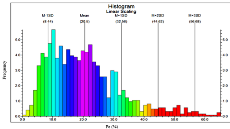
Fig. 3. Histogram of Fe concentration in drillcore samples of Central block in the North Anomaly deposit
