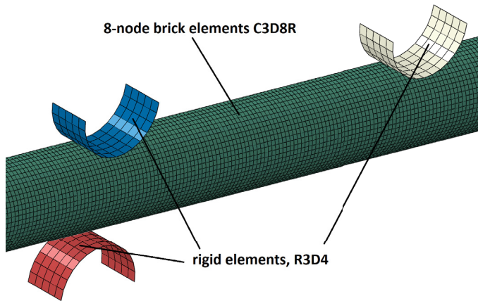
Fig. 7. A part of the finite element mesh
