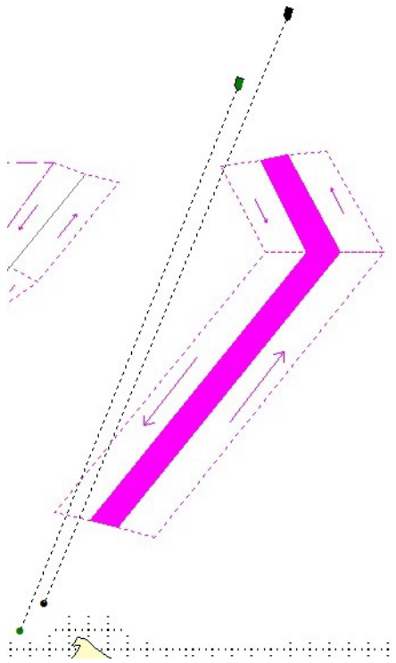
Figure 8. Initial parameters of ships from Scenario 5, speeds left to right: 15 and 18 knots
