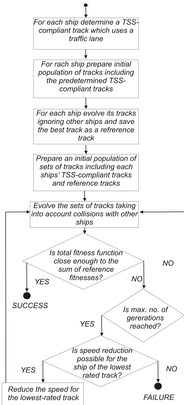
Figure 1. The ESoSST method's main algorithm including the use of reference tracks and reference fitness values.
