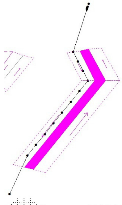
Figure 11. A reference track of the faster of the two ships in Scenario 3.
