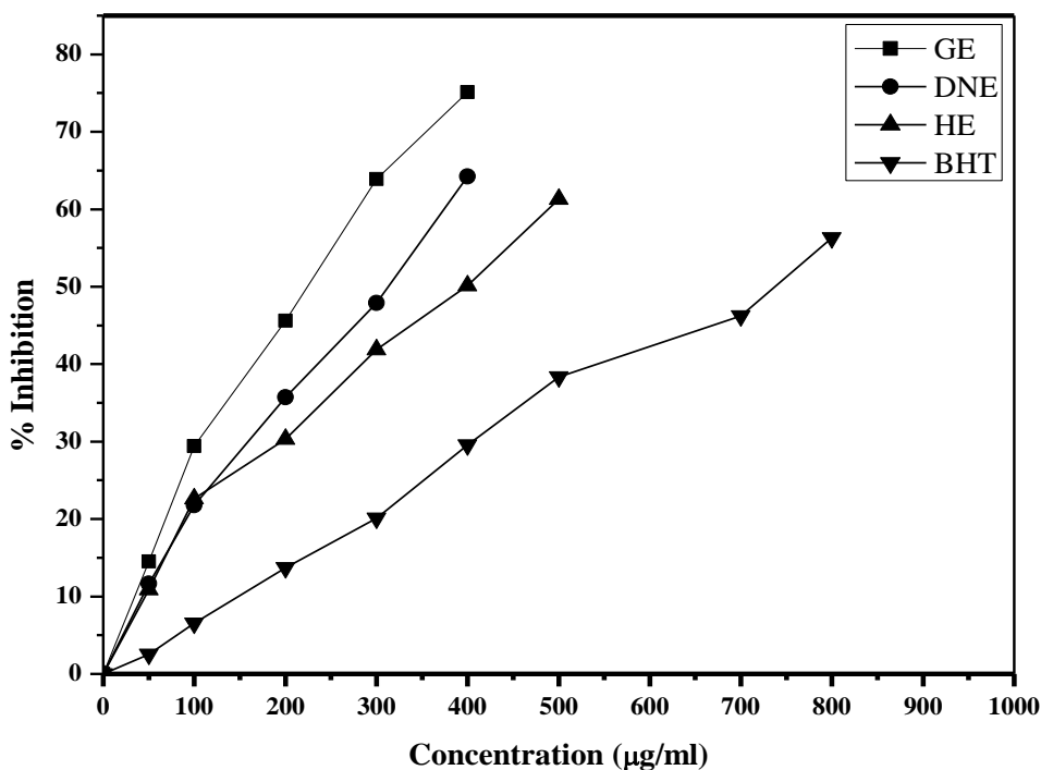
Fig. 4. Nitric oxide scavenging activities of ethanolic extract of selected varieties from Phoenix in comparison with BHT. Results were presented as mean \pm SD (n = 3).
