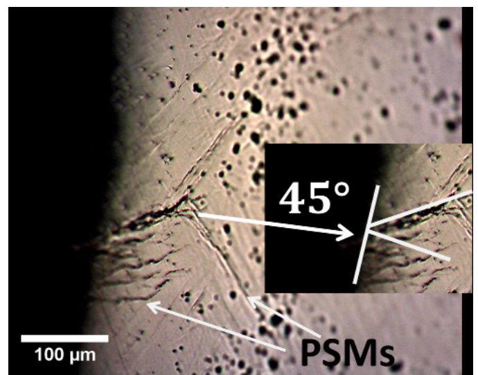
Fig. 9. Start of crack growth. Specimen charged with hydrogen
