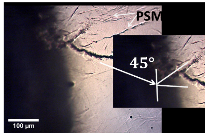
Fig. 8. Start of crack growth. Specimen without charge of hydrogen
