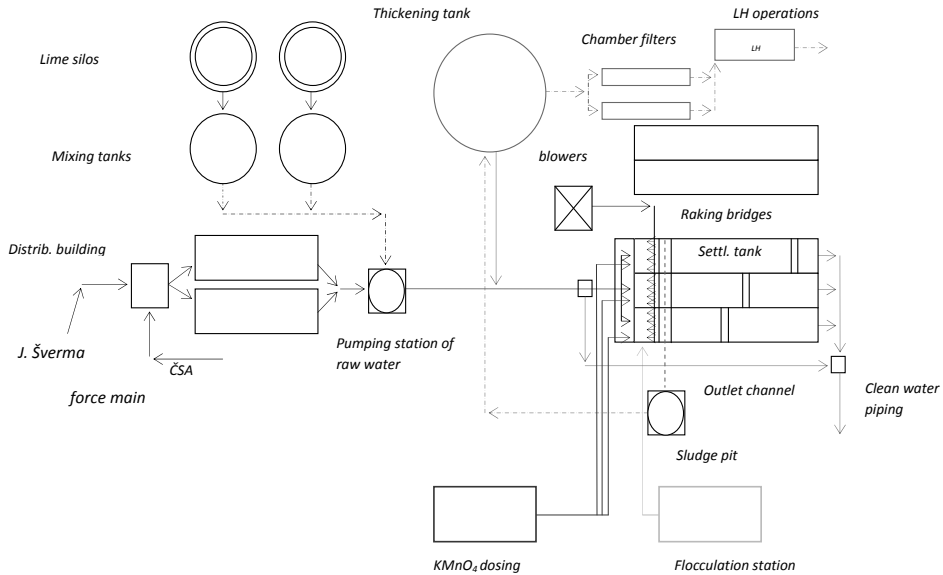
Fig. 1. Process diagram of the mine water treatment plant of the Coal Quarries ČSA and Jana Švermy [9]
