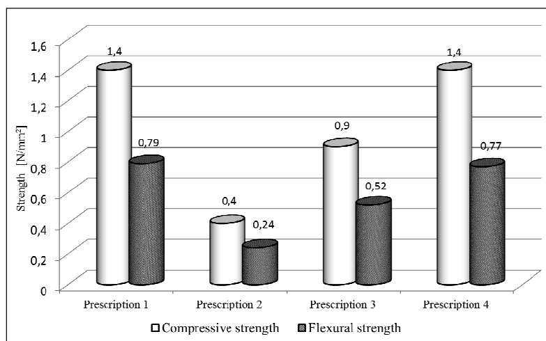
Fig. 2. Graphical representation of strength characteristics of the experimental prescriptions
