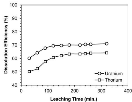
Fig. 4. Effect of leaching time on the dissolution efficiency of uranium and thorium from the fly ash sample (1.18 mmol/dm 3 HCl, 30% solid concentration, temperature 20 °C, pH~2.81)
