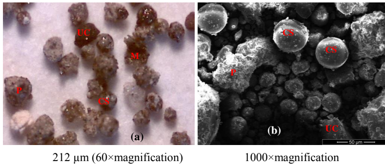
Fig. 2. Optical microscope and SEM photographs of fly ashes samples UC: unburned carbon, P: pozzolan, CS: cenosphere, M: magnetite
