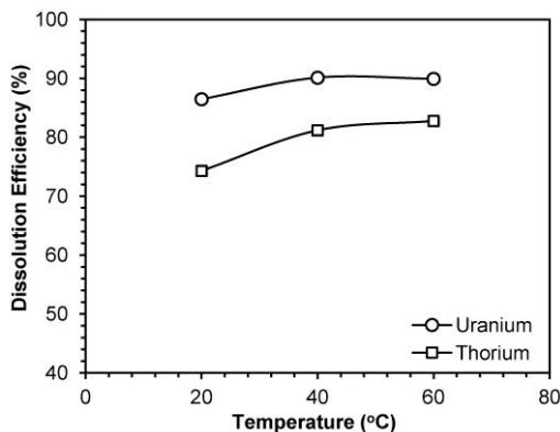
Fig. 6. Effect of temperature on dissolution efficiency of uranium and thorium from the fly ash sample (2.36 mmol/dm 3 HCl, 30% solid concentration, 240 min leaching time, pH~2.77)
