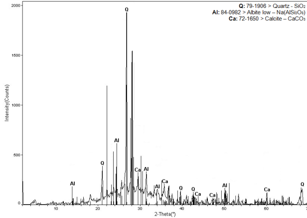
Fig. 1. XRD diffraction pattern of the fly ash sample
