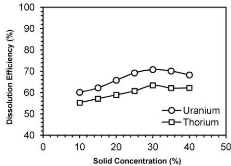
Fig. 3. Effect of solid concentration on dissolution efficiency of uranium and thorium from the fly ash sample (1.18 mmol/dm 3 HCl, 240 min leaching time at 20 °C, pH~2.79)
