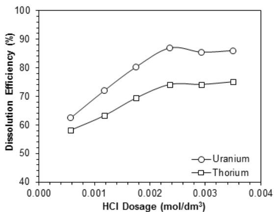
Fig. 5. Effect of reagent dosage on dissolution efficiency of uranium and thorium from the fly ash sample (30% solid concentration, 240 min leaching time, temperature 20 °C)
