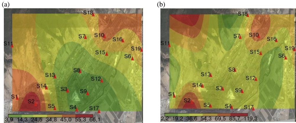
Fig. 3. GIS maps of air pollution in the area of El-Hadjar metallurgical plant; a) with Toluene, b) with Benzene
