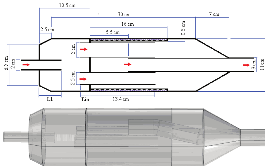
Fig. 11. Acoustical optimization in case I.
