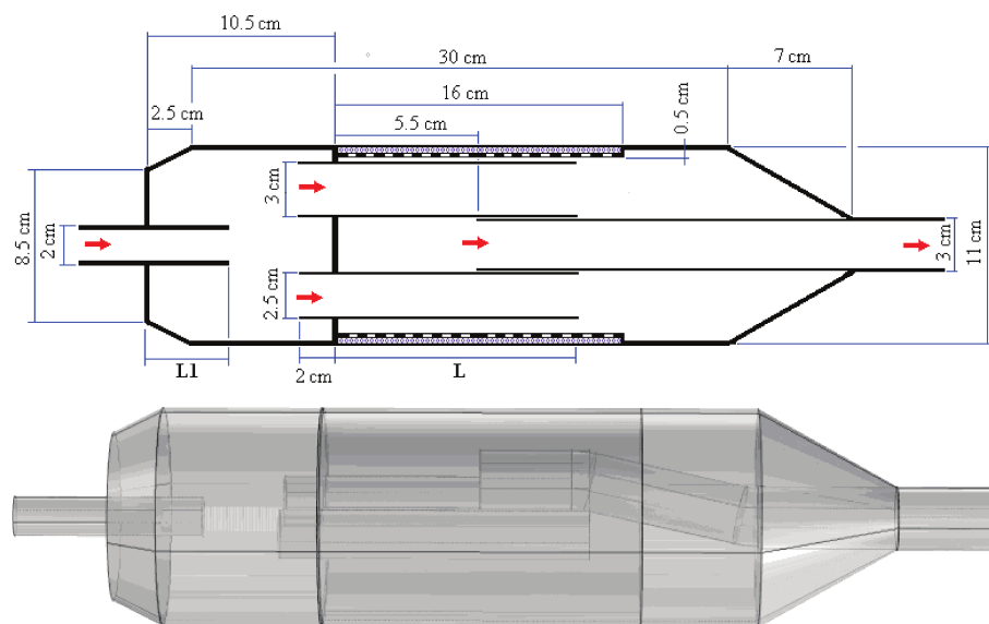
Fig. 12. Acoustical optimization in case II.
