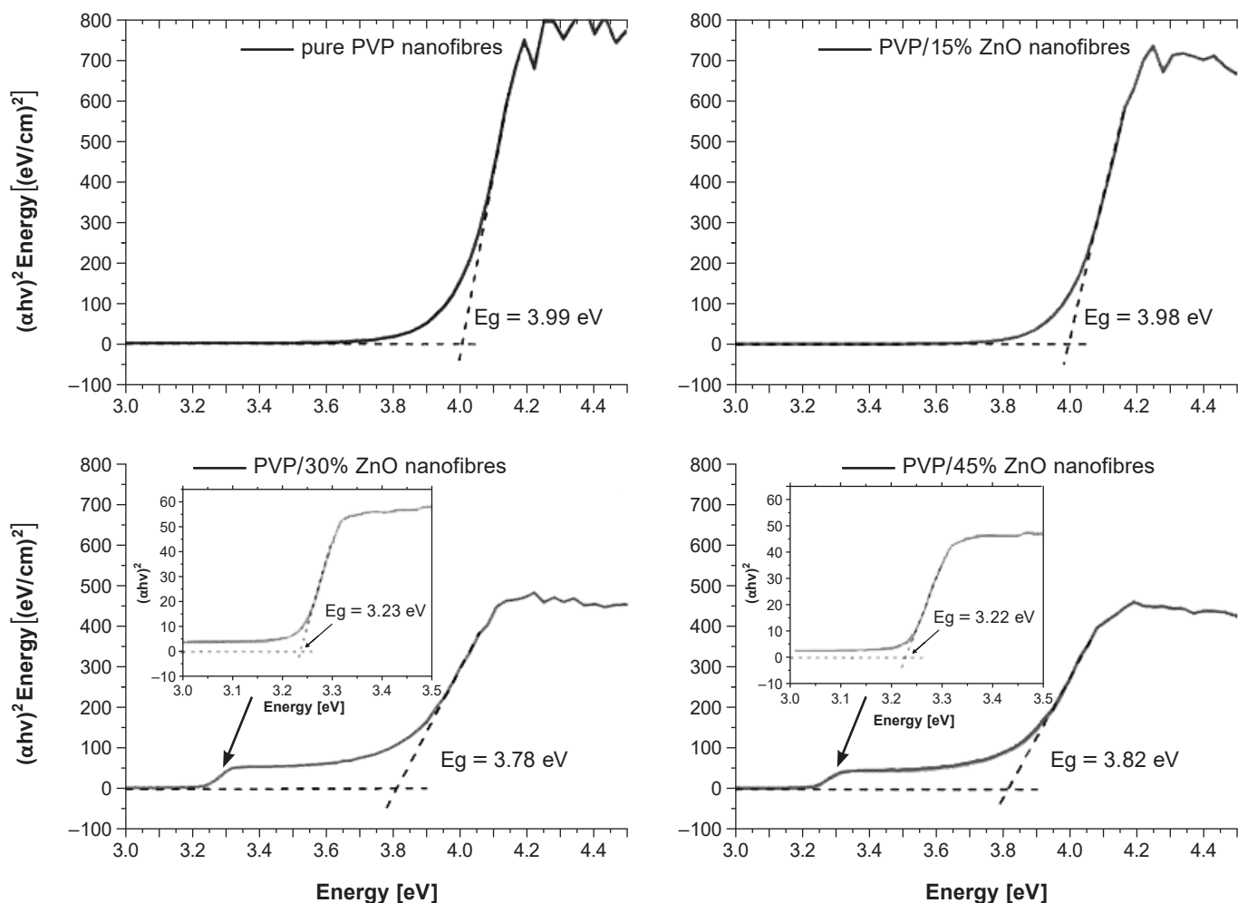
Fig. 8. Dependence (\alpha h\nu)^2 as function of quantum energy radiation determined based on UV-Vis spectra for the produced materials, and matching based on the smallest square method straight lines that define the zeros of linear functions corresponding to the band gap value
