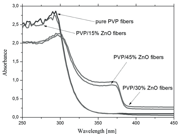
Fig. 7. UV-Vis spectrum for PVP and PVP/ZnO nanofibers
