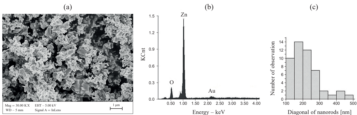
Fig. 1. a) SEM image of ZnO nanopowder, b) EDS analysis of the chemical composition of ZnO nanopowder (the presence of the gold peak is attributed to the conductive layer sprayed onto the fibrous mats to improve conductivity during the SEM examination), c) histogram showing the distribution of the diagonal values of the studied ZnO nanostructures
