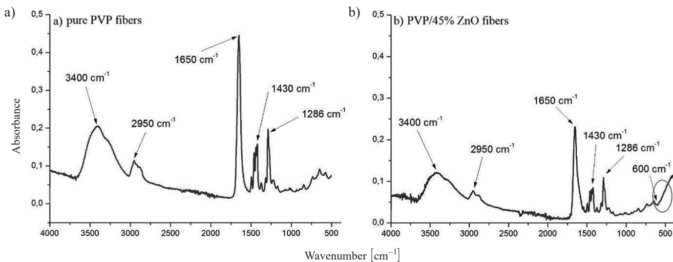
Fig. 6. FTIR spectra for: a) pure PVP nanofibers, b) PVP/45% ZnO composite nanofibers
