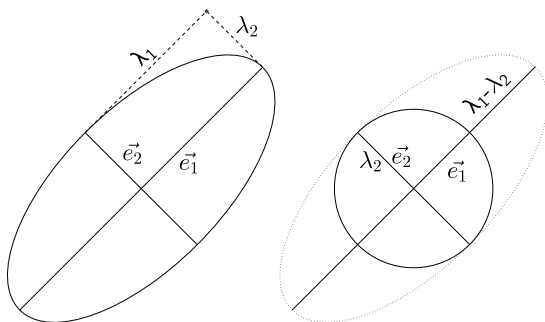
Fig. 4. Tensor decomposition.
