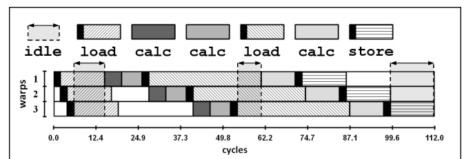
Fig. 7. Kernel program variant 1 from Listing 1 warps execution profile for a single core package within an SM
