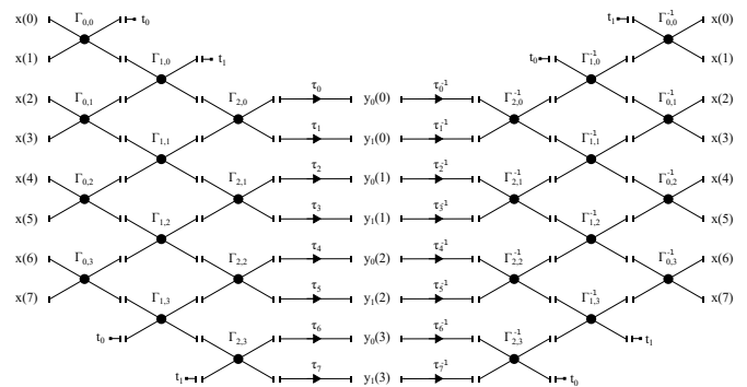
Fig. 1. Lattice structures of forward and inverse DWTs for transform size N = 8 and filter length K = 6
