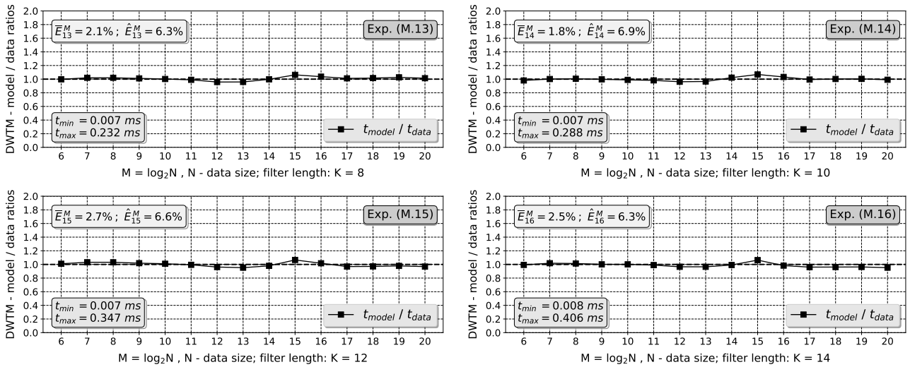
Model vs. data DWT Lattice algorithms execution times comparisons for GeForce GTX 1070 GPU (CUDA compute capability: 6.1 )
