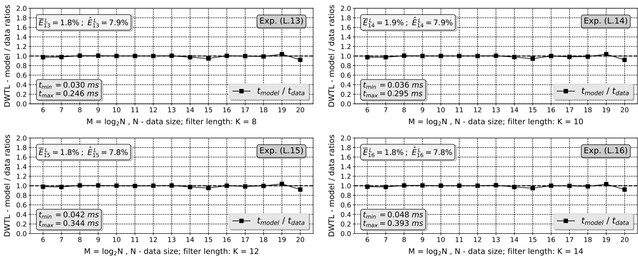
Model vs. data DWT matrix to DWT lattice execution times ratios for GeForce GTX 1070 GPU (CUDA compute capability: 6.1 )
