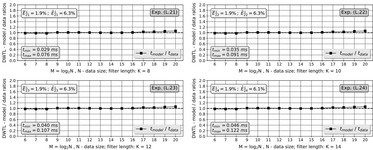
Model vs. data DWT matrix to DWT lattice execution times ratios for GeForce RTX 2080 GPU (CUDA compute capability: 7.5 )
