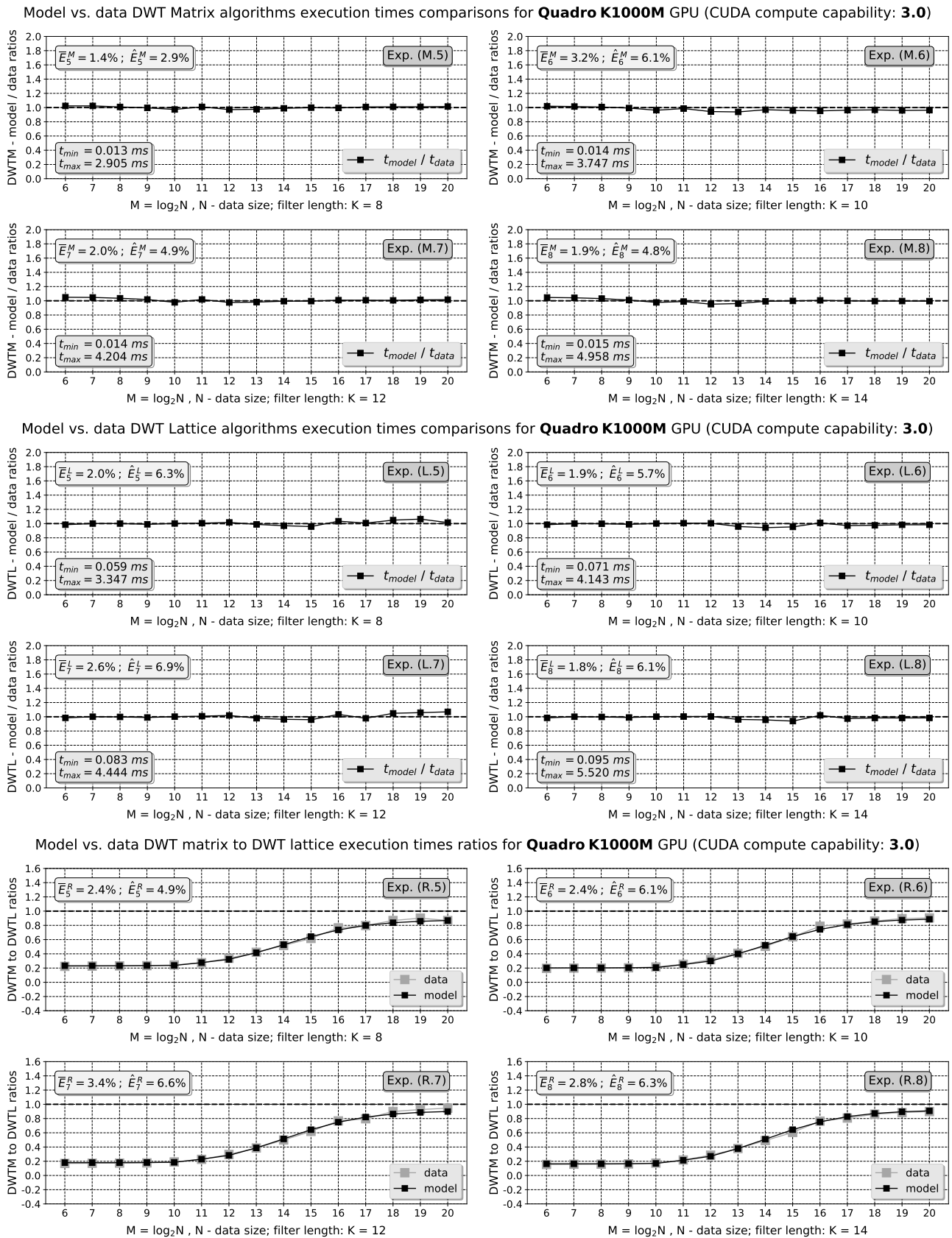
Fig. 11. Experimental results for Quadro K1000M GPU with DWT input data sizes M = 2^6, \dots, 2^{20} and filter lengths K \in \{8, 10, 12, 14\} . Experiments (M.5)–(M.8): DWT matrix algorithm modeled to measured execution times ratios. Experiments (L.5)–(L.8): DWT lattice algorithm modeled to measured execution times ratios. Experiments (R.5)–(R.8): DWT matrix to DWT lattice algorithms modeled to measured execution times ratios
