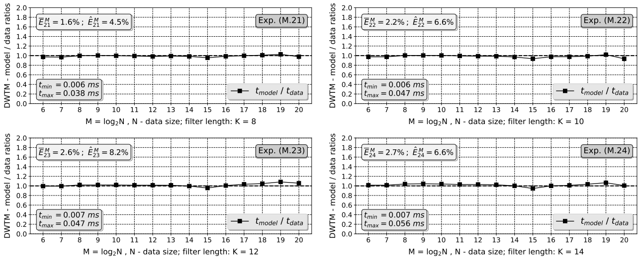
Model vs. data DWT Lattice algorithms execution times comparisons for GeForce RTX 2080 GPU (CUDA compute capability: 7.5 )
