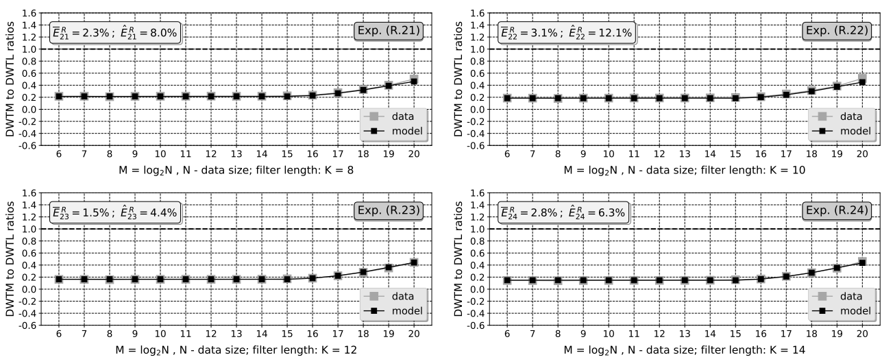
Fig. 15. Experimental results for GeForce RTX 2080 GPU with DWT input data sizes M = 2^6, \dots, 2^{20} and filter lengths K \in \{8, 10, 12, 14\} . Experiments (M. 21)–(M. 24): DWT matrix algorithm modeled to measured execution times ratios. Experiments (L. 21)–(L. 24): DWT lattice algorithm modeled to measured execution times ratios. Experiments (R. 21)–(R. 24): DWT matrix to DWT lattice algorithms modeled to measured execution times ratios
