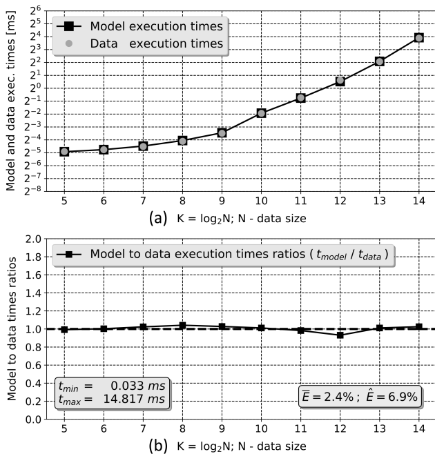
Fig. 9. Results obtained after final adjustment of all mt_x_mul_vec kernel program parameters – Listing 4, (a) modeled and measured overall execution times [ms], (b) modeled to measured execution times ratios
