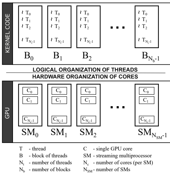
Fig. 4. Comparison of the logical organization of threads and GPU hardware construction
