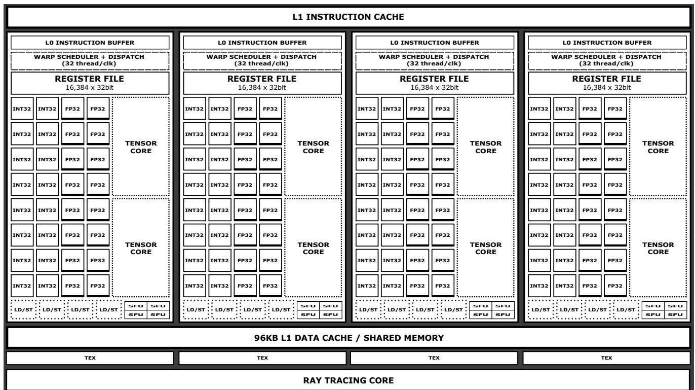
Fig. 5. Simplified scheme of a Streaming Multiprocessor built in CUDA 7.5 Compute Capability (Turing TU102/104/106)
