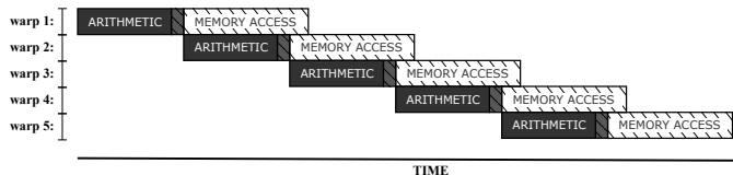
Fig. 6. Example of partial latency hiding by warp switching in an SM
