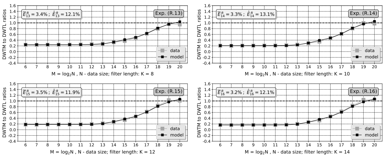
Fig. 13. Experimental results for GeForce GTX 1070 GPU with DWT input data sizes M = 2^6, \dots, 2^{20} and filter lengths K \in \{8, 10, 12, 14\} . Experiments (M. 13)–(M. 16): DWT matrix algorithm modeled to measured execution times ratios. Experiments (L. 13)–(L. 16): DWT lattice algorithm modeled to measured execution times ratios. Experiments (R. 13)–(R. 16): DWT matrix to DWT lattice algorithms modeled to measured execution times ratios
