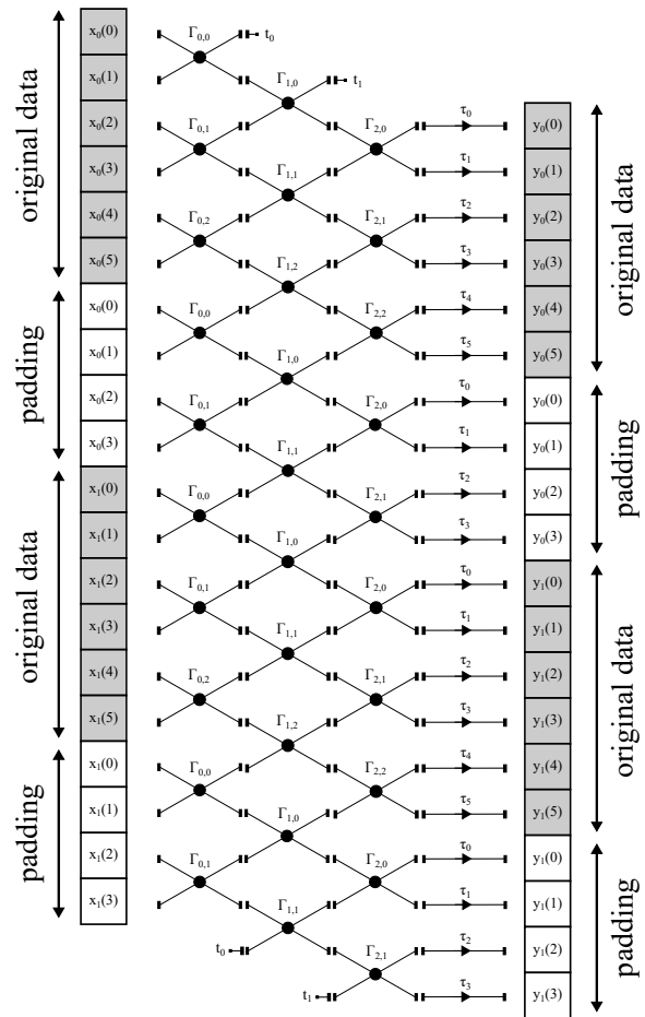
Fig. 2. Rows stage of 2D DWT row-column calculation using 1D lattice-structured DWT data flow graph with filter length K = 6 for 2 \times 6 - element input matrix padded with K - 2 cyclic element repetition
