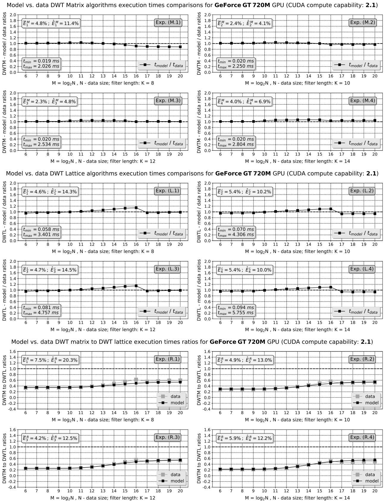
Fig. 10. Experimental results for GeForce GT 720M GPU with DWT input data sizes M = 2^6, \dots, 2^{20} and filter lengths K \in \{8, 10, 12, 14\} . Experiments (M. 1)–(M. 4): DWT matrix algorithm modeled to measured execution times ratios. Experiments (L. 1)–(L. 4): DWT lattice algorithm modeled to measured execution times ratios. Experiments (R. 1)–(R. 4): DWT matrix to DWT lattice algorithms modeled to measured execution times ratios
