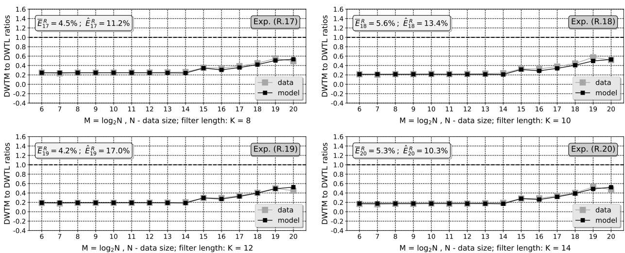
Fig. 14. Experimental results for GeForce RTX 2060 GPU with DWT input data sizes M = 2^6, \dots, 2^{20} and filter lengths K \in \{8, 10, 12, 14\} . Experiments (M. 17)–(M. 20): DWT matrix algorithm modeled to measured execution times ratios. Experiments (L. 17)–(L. 20): DWT lattice algorithm modeled to measured execution times ratios. Experiments (R. 17)–(R. 20): DWT matrix to DWT lattice algorithms modeled to measured execution times ratios
