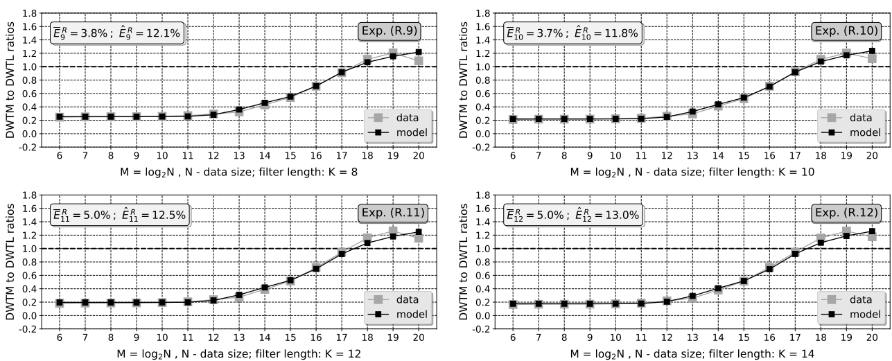
Fig. 12. Experimental results for GeForce GTX 860M GPU with DWT input data sizes M = 2^6, \dots, 2^{20} and filter lengths K \in \{8, 10, 12, 14\} . Experiments (M. 9)–(M. 12): DWT matrix algorithm modeled to measured execution times ratios. Experiments (L. 9)–(L. 12): DWT lattice algorithm modeled to measured execution times ratios. Experiments (R. 9)–(R. 12): DWT matrix to DWT lattice algorithms modeled to measured execution times ratios
