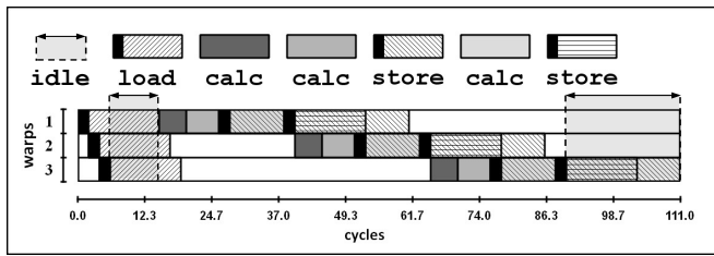
Fig. 8. Kernel program variant 2 from Listing 1 warps execution profile for a single core package within an SM
