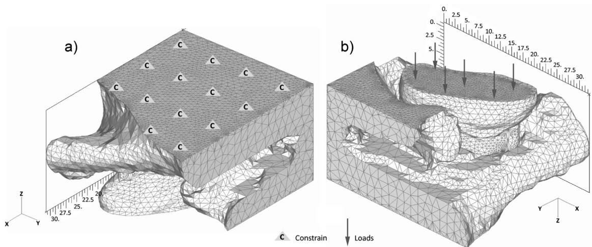
Fig. 4. Numeric model of TMJ with preset: a) constrain, b) loads [L. 15]
