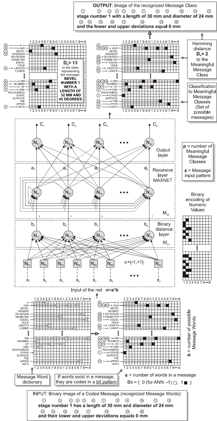
Fig. 6. General concept of message recognition using neural networks
