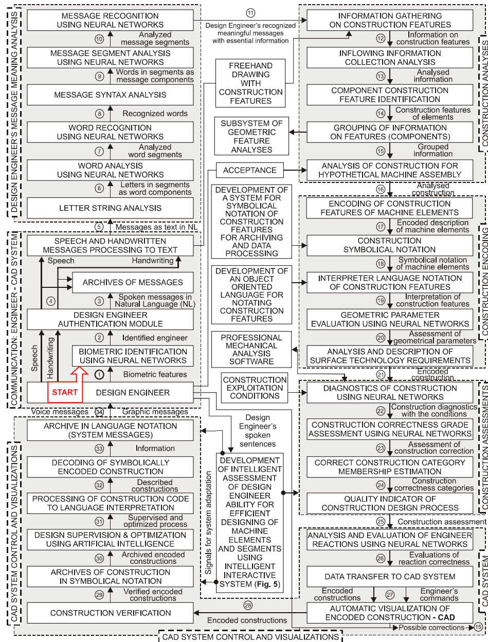
Fig. 4. The general concept of interactive automated design of machine elements and assemblies [1]
