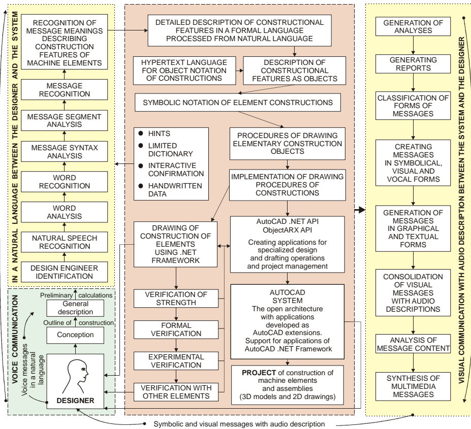
Fig. 2. Concept of interactive design of machine elements and assemblies
