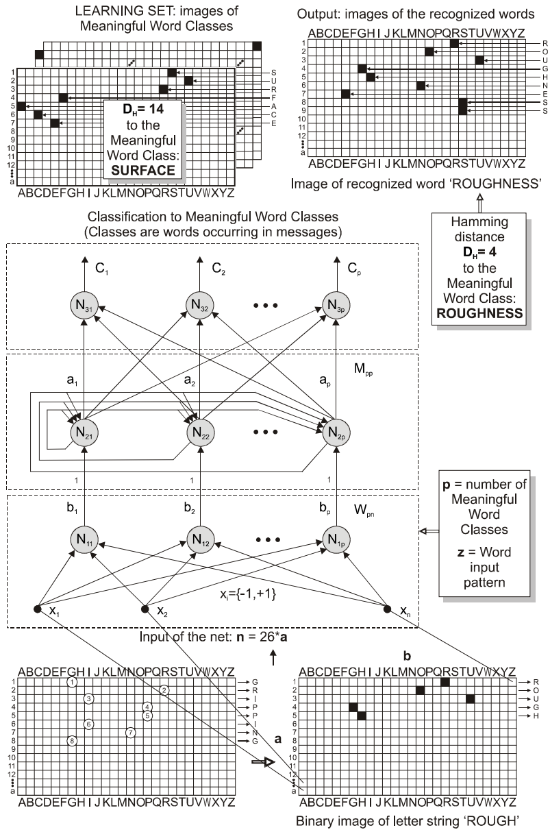
Fig. 5. General concept of word recognition using neural networks [11]
