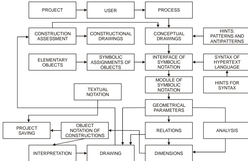
Fig. 1. Concept of automated design of machine elements and assemblies
