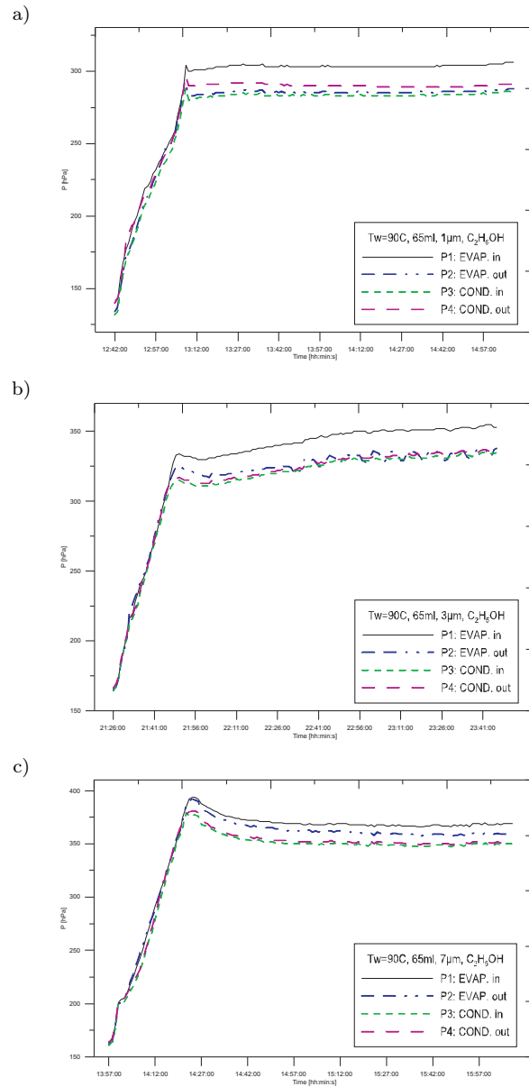
Figure 11: Pressure distribution in function of time in four specific nodes of installation. Working fluid-ethanol, T_w = 90 \text{ }^\circ\text{C} , filling volume 65 ml, pore size a) d_p = 1 \mu m , b) d_p = 3 \mu m , c) d_p = 7 \mu m .
