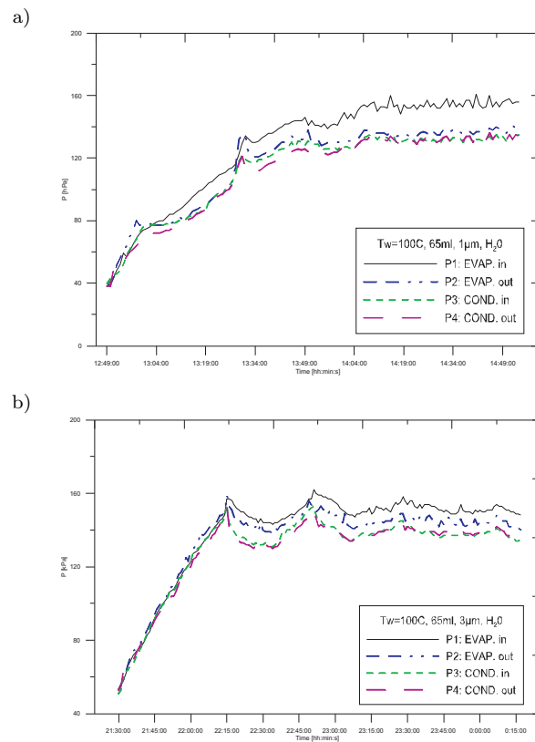
Figure 9: Pressure distribution in function of time in four specific nodes of installation. Working fluid-water, T_w = 100\text{ }^\circ\text{C} , filling volume 65 ml, pore size a) d_p = 1\ \mu\text{m} , b) d_p = 3\ \mu\text{m} .
