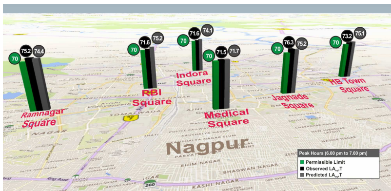
Fig. 5. Comparative analysis of permissible limit, observed and predicted L_{Aeq} during peak hours (6.00 pm to 7.00 pm).
