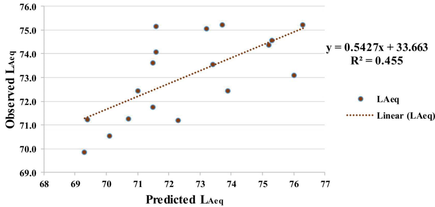
Fig. 9. Correlation between observed and predicted L_{Aeq, T} for morning, afternoon and night hours.
