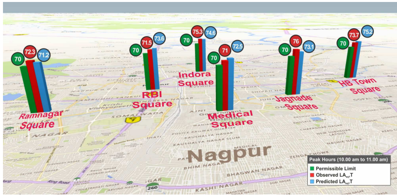
Fig. 3. Comparative analysis of permissible limit, observed and predicted L_{Aeq} during peak hours (10.00 am to 11.00 am).
