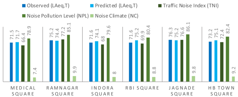
Fig. 8. Comparative analysis of observed and predicted L_{Aeq,T} with noise pollution parameters during peak hours (6.00 pm to 7.00 pm).
