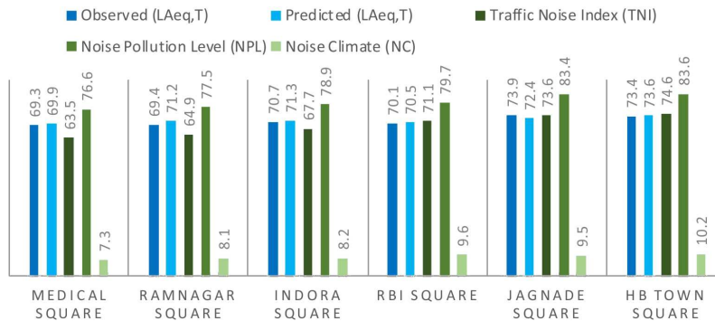
Fig. 7. Comparative analysis of observed and predicted L_{Aeq,T} with noise pollution parameters during non-peak hours (2.30 am to 3.30 am).
