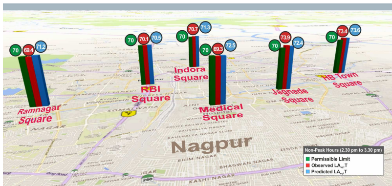
Fig. 4. Comparative analysis of permissible limit, observed and predicted L_{Aeq} during non-peak hours (2.30 am to 3.30 am).
