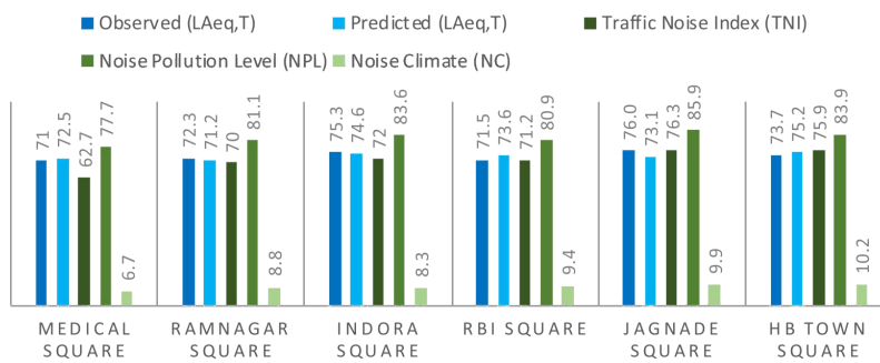
Fig. 6. Comparative analysis of observed and predicted L_{Aeq,T} with noise pollution parameters during peak hours (10.00 am to 11.00 am).
