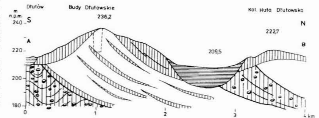
Fig. 4. Budy Dłutowskie. An example of glaciotectionic pair: depression-elevation. A – hypsometric sketch with the axes of depression (broken line) and elevation (solid line), and the A-B cross-section line; B – simplified geological cross-section along the A-B line: 1 – older till; 2 – younger till, glaciotectionically displaced; 3 – glaciofluvial deposits; 4 – glaciolacustrine sandy-silty deposits.
