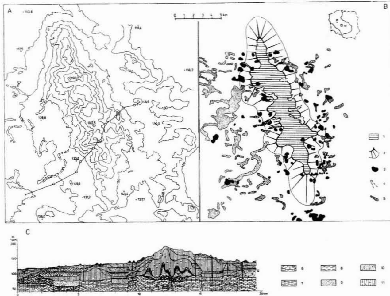
Fig. 3. The Malanów Ridge – an example of a continuous ridge form with glaciotectionic structure. A – hypsometric sketch and the line of geological cross-section; B – morphologic sketch: 1 – ridge surface made up largely of till; 2 – scarps and distinct slopes; 3 – kame hillocks at the foot and on the slopes; 4 – small denudational valleys; 5 – major dune complexes; C – geological cross-section along the A-B line (after Mańkowska, 1987, generalised): 6 – limestones, marls and opokas; 7 – clays; 8 – silts; 9 – sands; 10 – glaciofluvial sands with gravels; 11 – tills.
