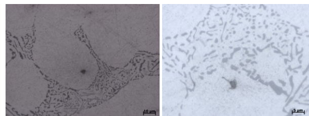
Fig. 4, 5. Inclusions in primary \alpha(\text{Al}) phase observed by light microscopy
