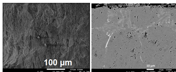
Fig. 2, 3. Inclusions in structure observed by electron microscopy
