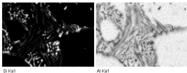
Fig. 8, 9. Mapping for silicon (left) and aluminium (right)
