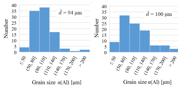
Fig. 23, 24. Average grain size – no inoculation (left), 0,05 % AlTi5B1 (right)
