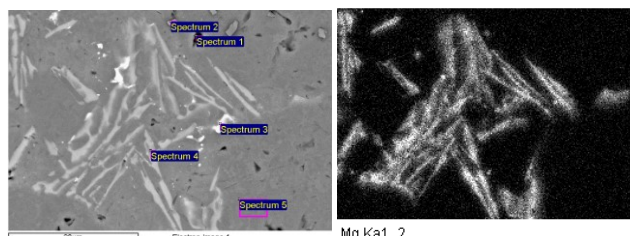
Fig. 6, 7. Studied structure (left) and mapping for magnesium (right)
