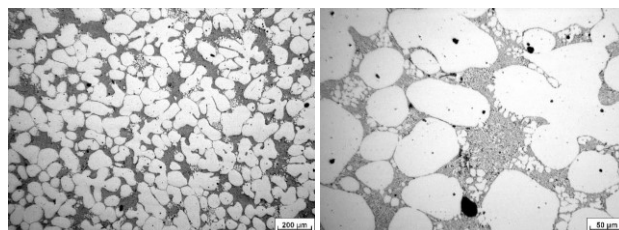
Fig. 18, 19. Structure inoculated by 0,15 % AlTi5B1
