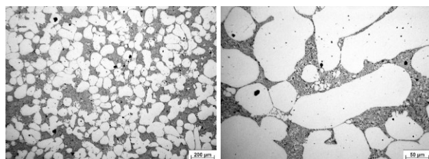
Fig. 16, 17. Structure inoculated by 0,1 % AlTi5B1
