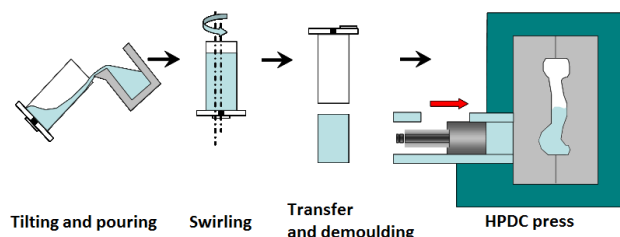
Fig. 1. SEED rheocasting method principle – phases [2]
