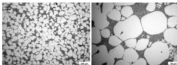
Fig. 20, 21. Structure inoculated by 0,2 % AlTi5B1
