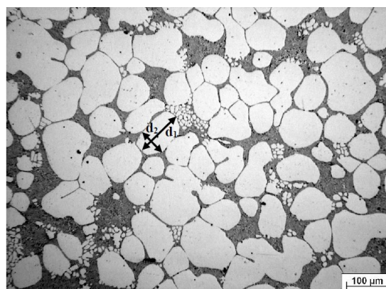
Fig. 22. Measuring of grain size
