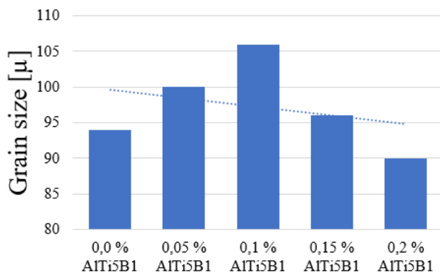
Fig. 28. Average grain size
