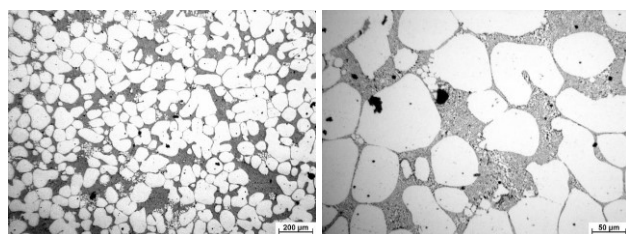
Fig. 12, 13. As cast structure without inoculation
