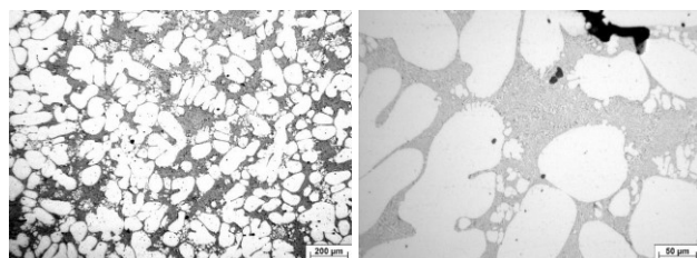
Fig. 14, 15. Structure inoculated by 0,05 % AlTi5B1
