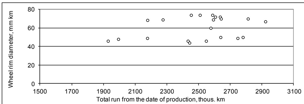
Fig. 5. The results of the probability research of M62 locomotive wheel rim diameter according to total run from the date of production
