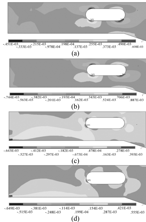
Fig.6. Deformation distribution in the strain concentrators [(a) Braking, Y direction, (b) Traction, Y direction. (c) Braking, Z direction and (d) Traction, Z direction]
