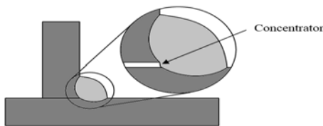
Fig.10. Stress concentrator on a fillet weld due to a gap between the two joint elements
