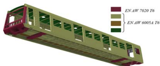
Fig. 8. Material composition of the car body of a Metro coach, built in 1980's
