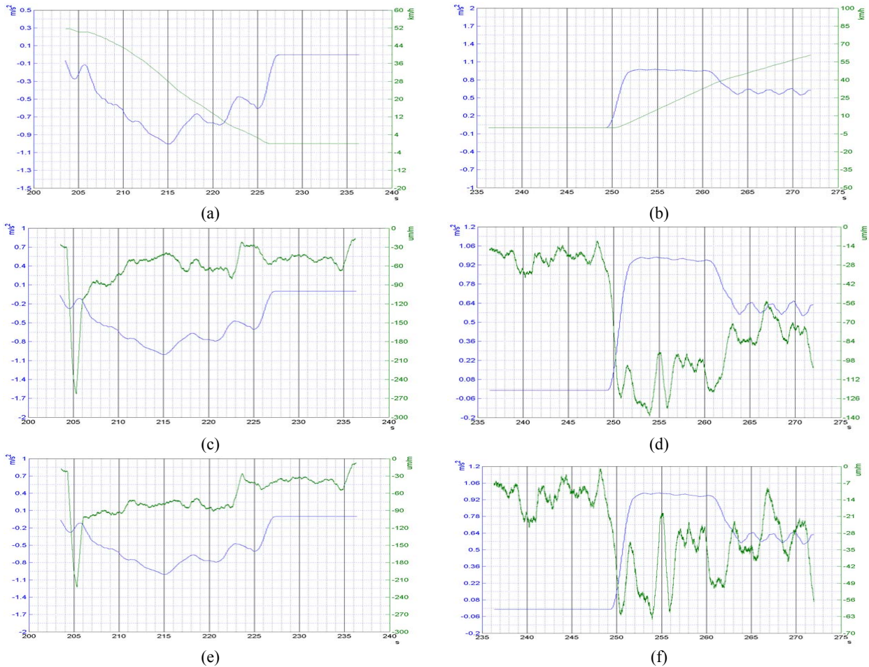
Fig.4. Signals in time domain - (a) Acceleration and velocity at entrance to the station, (b) Acceleration and velocity at exit the station, (c) D3T and acceleration at entrance to the station, (d) D3T and acceleration at exit the station, (e) D3V and acceleration at entrance to the station and (f) D3V and acceleration at exit the station
