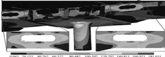
Fig. 5. Strain distribution (Von-Misses) [MPa]
