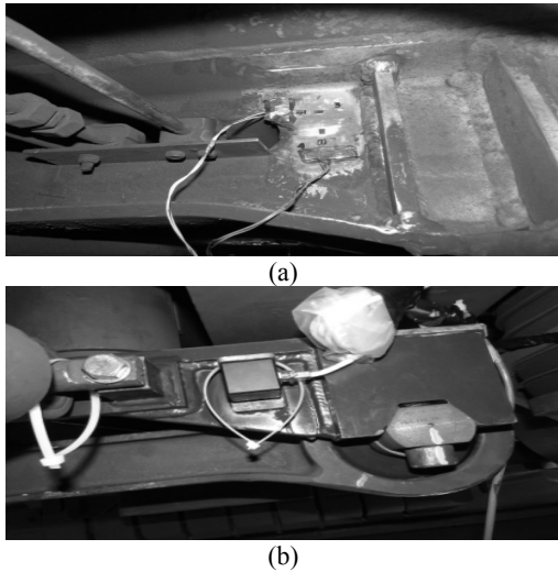
Fig.3. Location of sensors - (a) strain gauges, (b) tri-axial accelerometer
