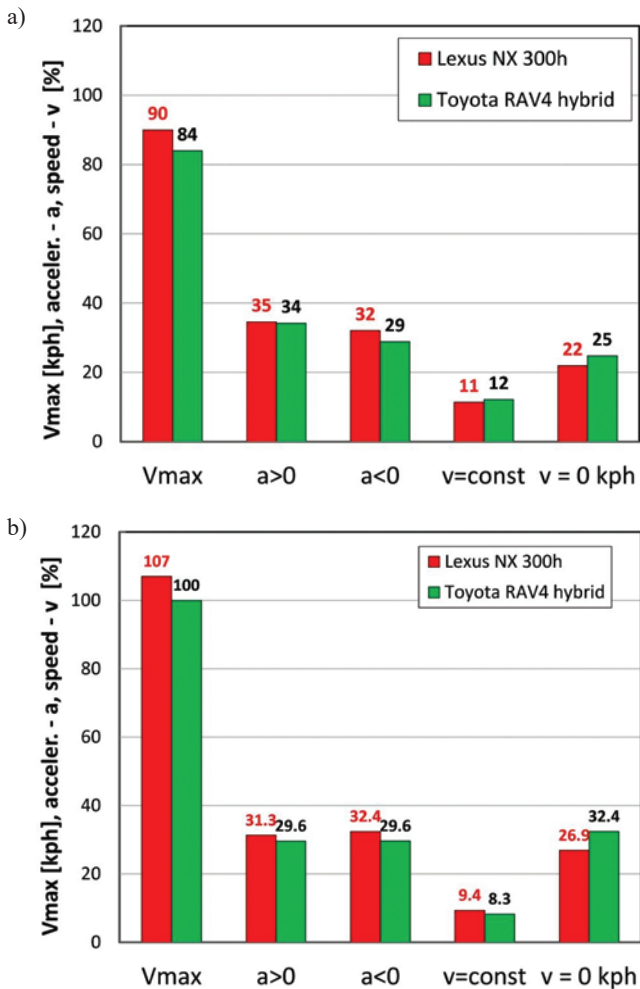
Fig. 3. Characteristic measured values of the test drives: a) in urban driving conditions, b) in non-urban driving conditions
