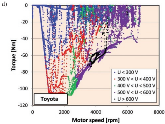
Fig. 5. Electric motor characteristics of the tested vehicles during regenerative braking: d) in non-urban driving conditions relative to the supply voltage
