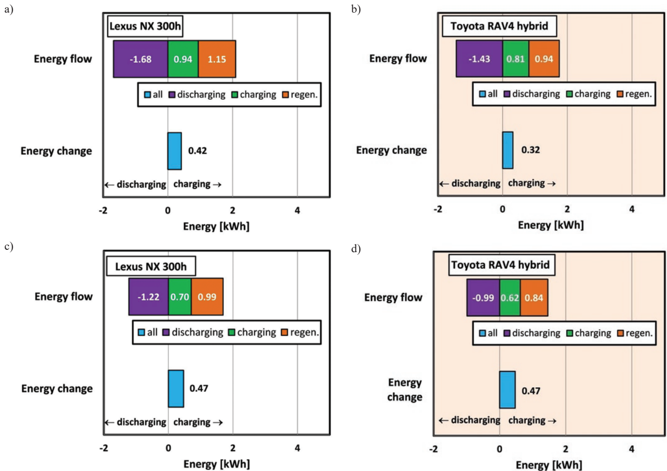
Fig. 9. The energy flow and total change of battery charge analysis during driving: a–b) in urban driving conditions, c–d) in non-urban driving conditions, including charging, high-voltage discharge and regenerative braking
