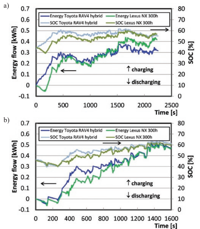
Fig. 7. Analysis of energy flow and battery charge of the vehicles during the drives: a) in urban driving conditions, b) in non-urban driving conditions
