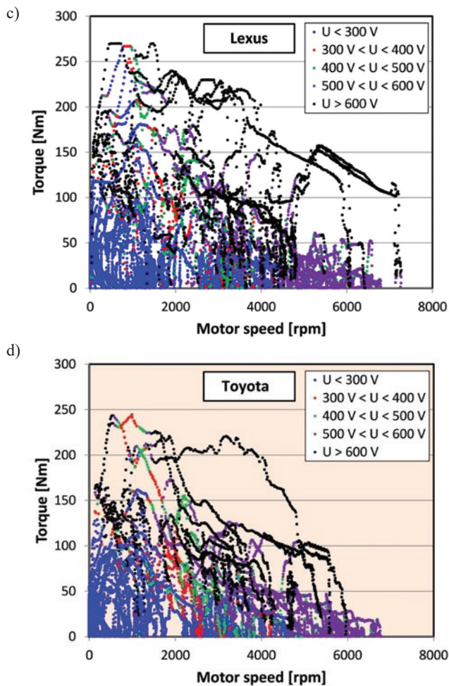
Fig. 4. Electric motors characteristics of the tested vehicles: c-d) in non-urban driving conditions relative to the supply voltage
