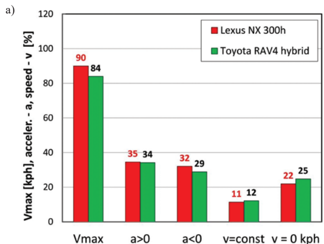
Fig. 2. Tested vehicles speed comparison: a) in urban driving conditions
