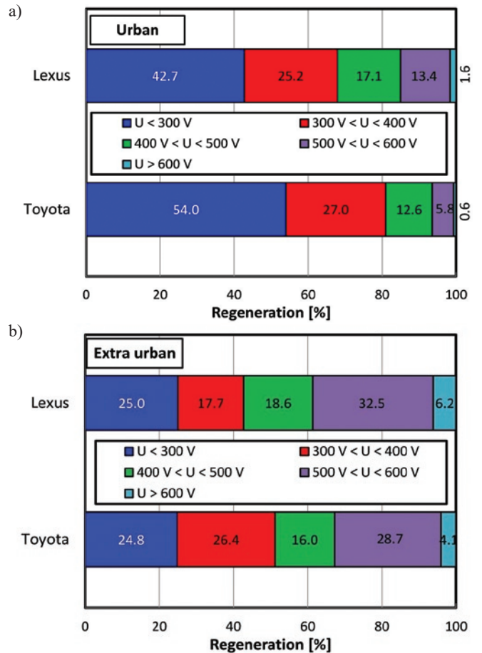
Fig. 6. Analysis of relative energy recovery time shares taking into account the electric generator voltage of the tested vehicles: a) in urban driving conditions, b) in non-urban driving conditions
