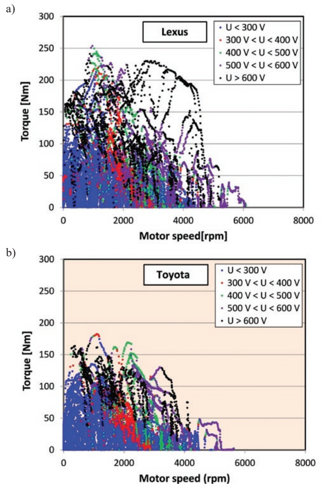
Fig. 4. Electric motors characteristics of the tested vehicles: a–b) in urban driving conditions relative to the supply voltage
