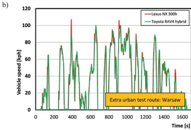
Fig. 2. Tested vehicles speed comparison: b) in non-urban driving conditions
