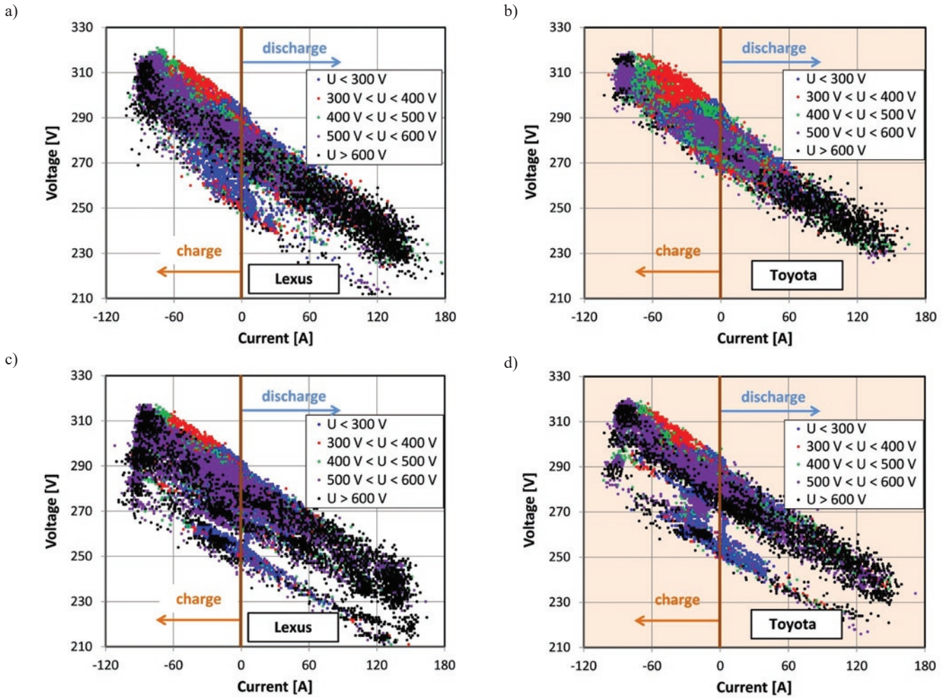
Fig. 8. Charging and discharging voltage characteristics of high-voltage batteries: a–b) in urban driving conditions, c–d) in non-urban driving conditions relative to the supply voltage of the electric motors
