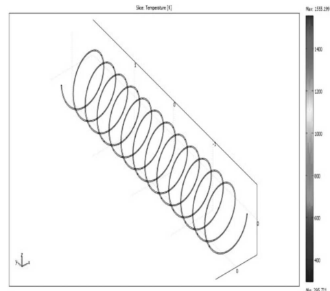
Fig. 5. Temperature distribution of TiN micro tubular heater coil
