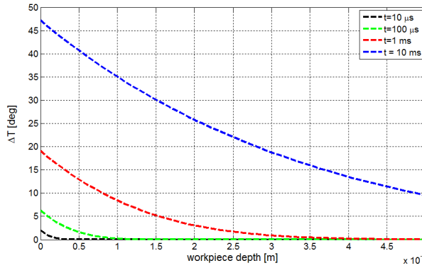
Fig. 15. Temperature rise in material depending on processing time for v=10mm/min and laser beam w_0=1,8mm
