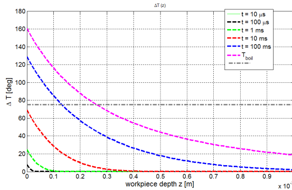
Fig. 14. Temperature rise in material, depending on processing time for v=10mm/min and laser beam w_0=0,9 mm
