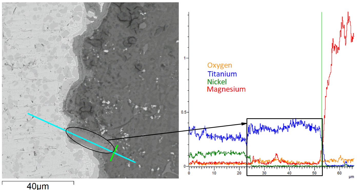
Fig. 5. Chemical analysis at the matrix-reinforcement interface
