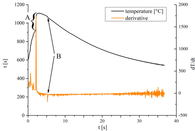
Fig. 1. SHS temperature-time dependence
