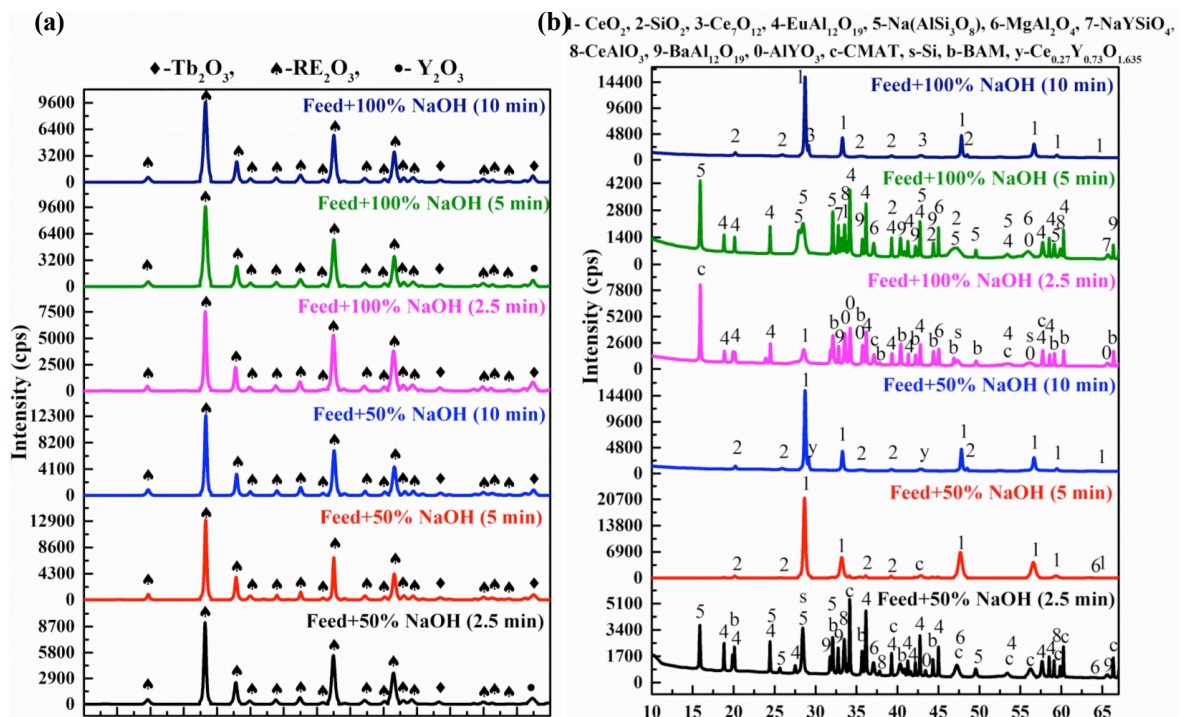
Fig. 12. XRD spectra of (a) rare earth oxides and (b) leach residues obtained from microwave exposure of feed with 50% and 100% NaOH for duration 2.5, 5, and 10 min
