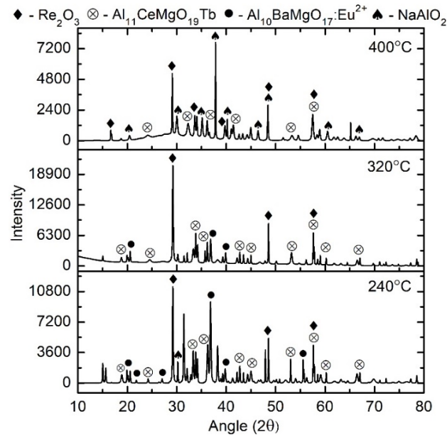
Fig. 5. XRD spectra of heat-treated products at different temperatures
