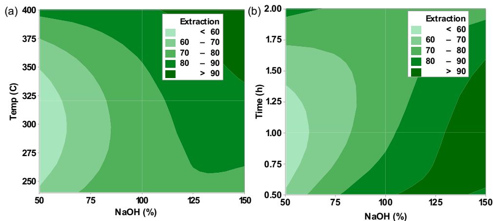
Fig. 4. Contour plots showing the response surfaces for flux dosage with (a) temperature (b) time
