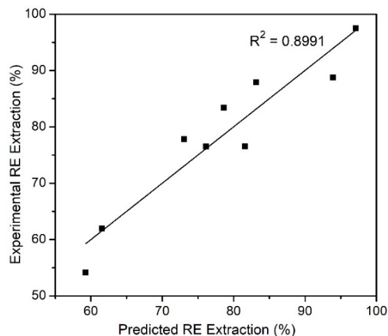
Fig. 6. Regression plot for experimental and predicted values for RE extraction
