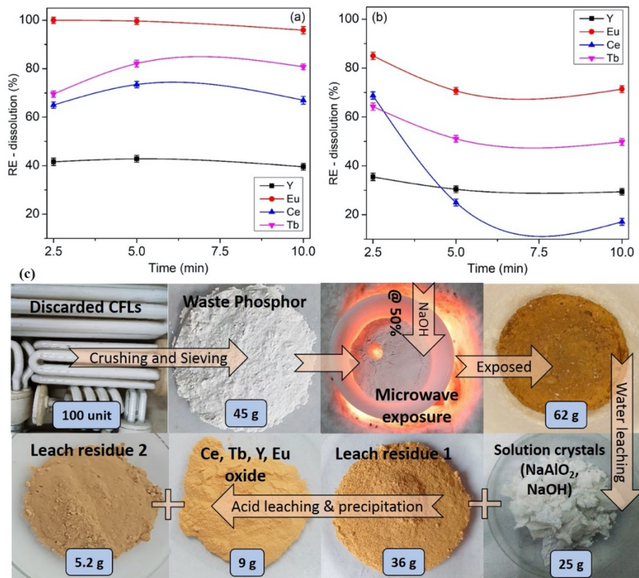
Fig. 11. Effect of microwave exposure on RE dissolution at (a) 50 % NaOH, (b) 100 % NaOH, (c) Material balance and sample specimen photographs (5 min microwave, 50 wt-% NaOH dosage)
