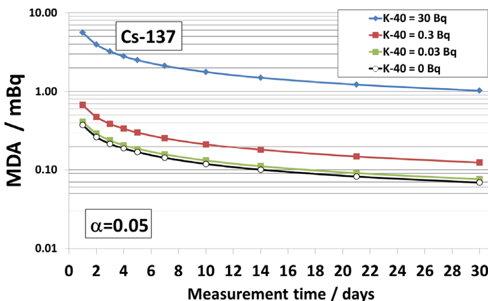
Fig. 5. Detection limits (MDA) for ^{137}\text{Cs} in a 4-g seawater precipitate sample, measured in a 2-kg well detector (Ge-12 in HADES), as a function of measurement time for different activities of ^{40}\text{K} in the sample.
