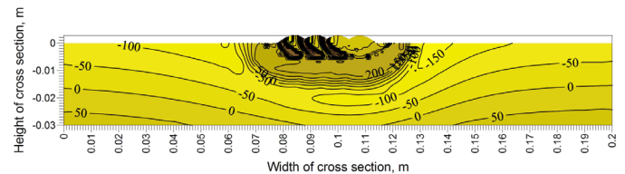
Fig. 19. The stress distribution in the whole cross section after application of 4th weld
