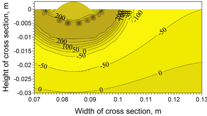
Fig. 14. The stress distribution in the middle part of cross section after application of 1st weld
