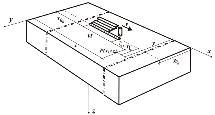
Fig. 1. The scheme of multi-pass weld surfacing: v – velocity of electrode; x_{0k} – coordinate of the beginning of k -th weld; y_{0k} – coordinate of k -th weld axis; t – time, that has elapsed since the beginning of surfacing, \xi_k and \eta_k – distances from considered point of the plate to the position of the electrode
