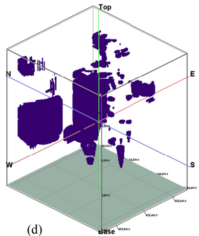
Fig. 7. RQD populations in the Kahang deposit based on thresholds defined from the RQD-N fractal model (a) very poor zones; (b) very poor & poor zones; (c) fair and good zones; (d) excellent zones
